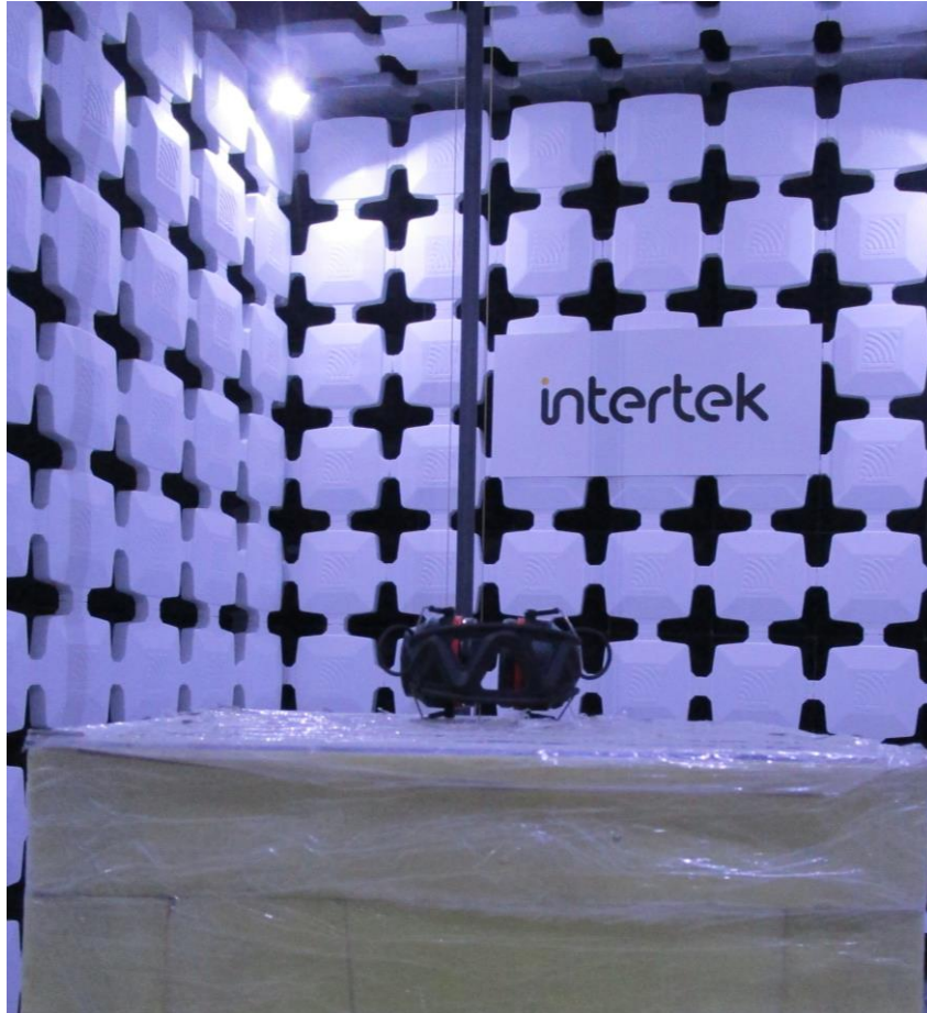
Above 1GHz The EUT is placed at the center of turntable
