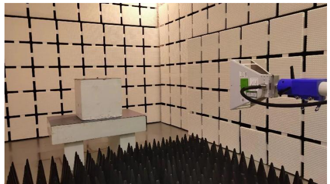
Radiated Emissions for 1GHz~5GHz
