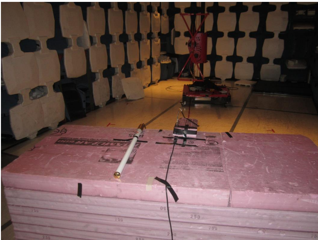
Radiated Emissions - 30 to 1000 MHz (w/ Laird Antenna)
