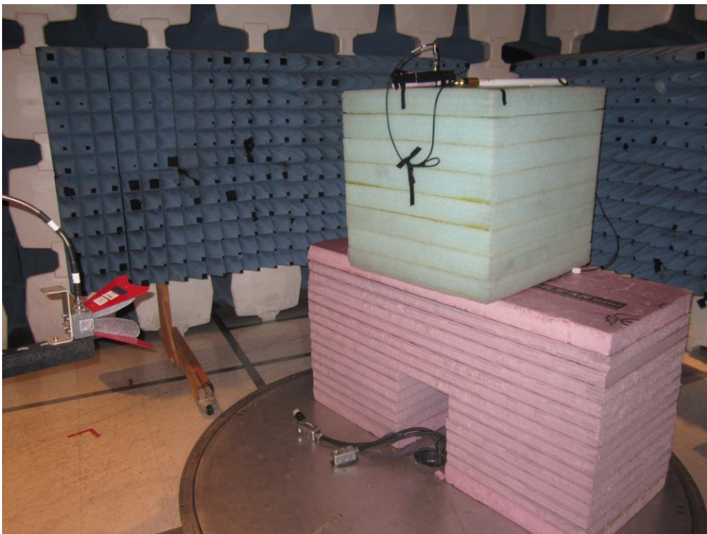
Radiated Emissions - 6 to 10 GHz (w/ Laird Antenna)
