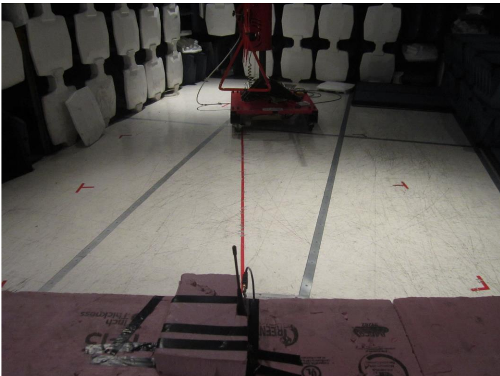
Radiated Emissions - 30 to 1000 MHz (w/ Nearson Antenna)
