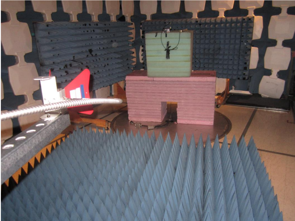
Radiated Emissions - 1 to 6 GHz (w/ Laird Antenna)
