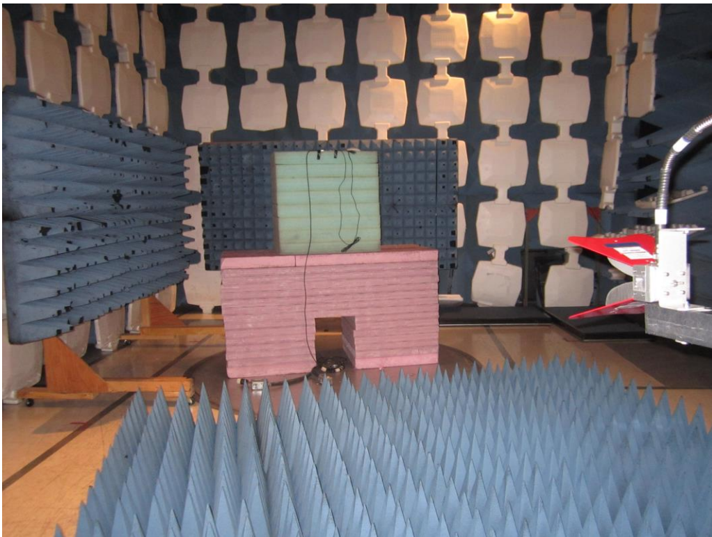
Radiated Emissions - 1 to 6 GHz (w/ Taoglas Antenna)
