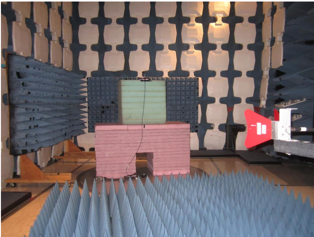
Radiated Emissions - 1 to 6 GHz (w/ LINX Antenna)
