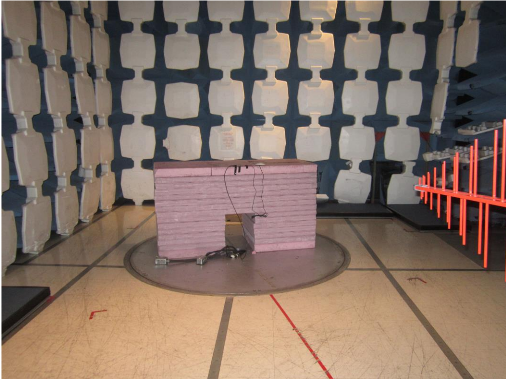
Radiated Emissions - 30 to 1000 MHz (w/ Taoglas Antenna)
