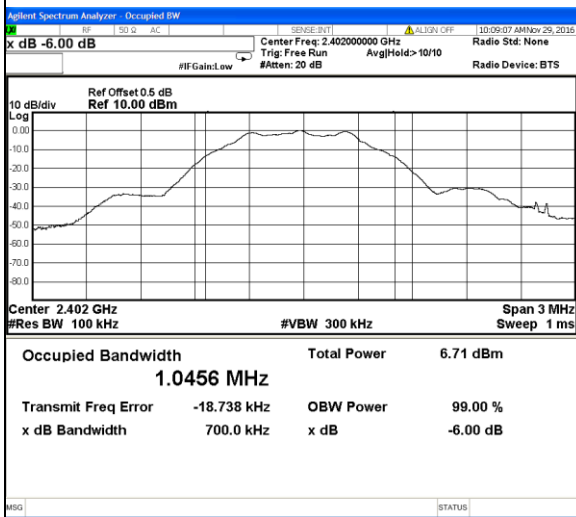
Channel 0 / 2402 MHz
