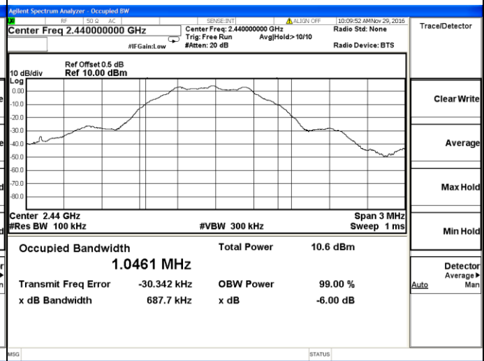
Channel 19 / 2440 MHz
