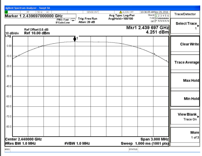
Channel 19 / 2440 MHz
