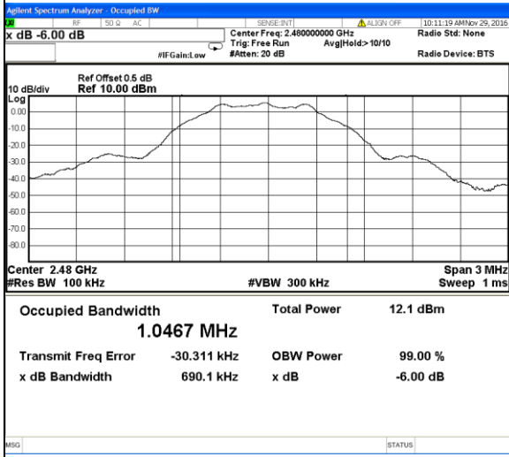
Channel 39 / 2480 MHz
