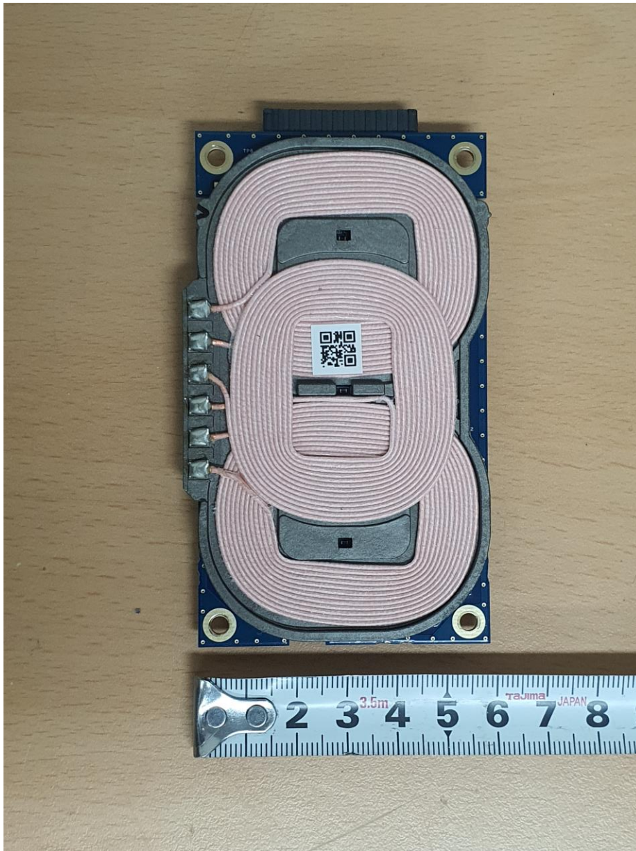
< Sub board bottom view #1 >
