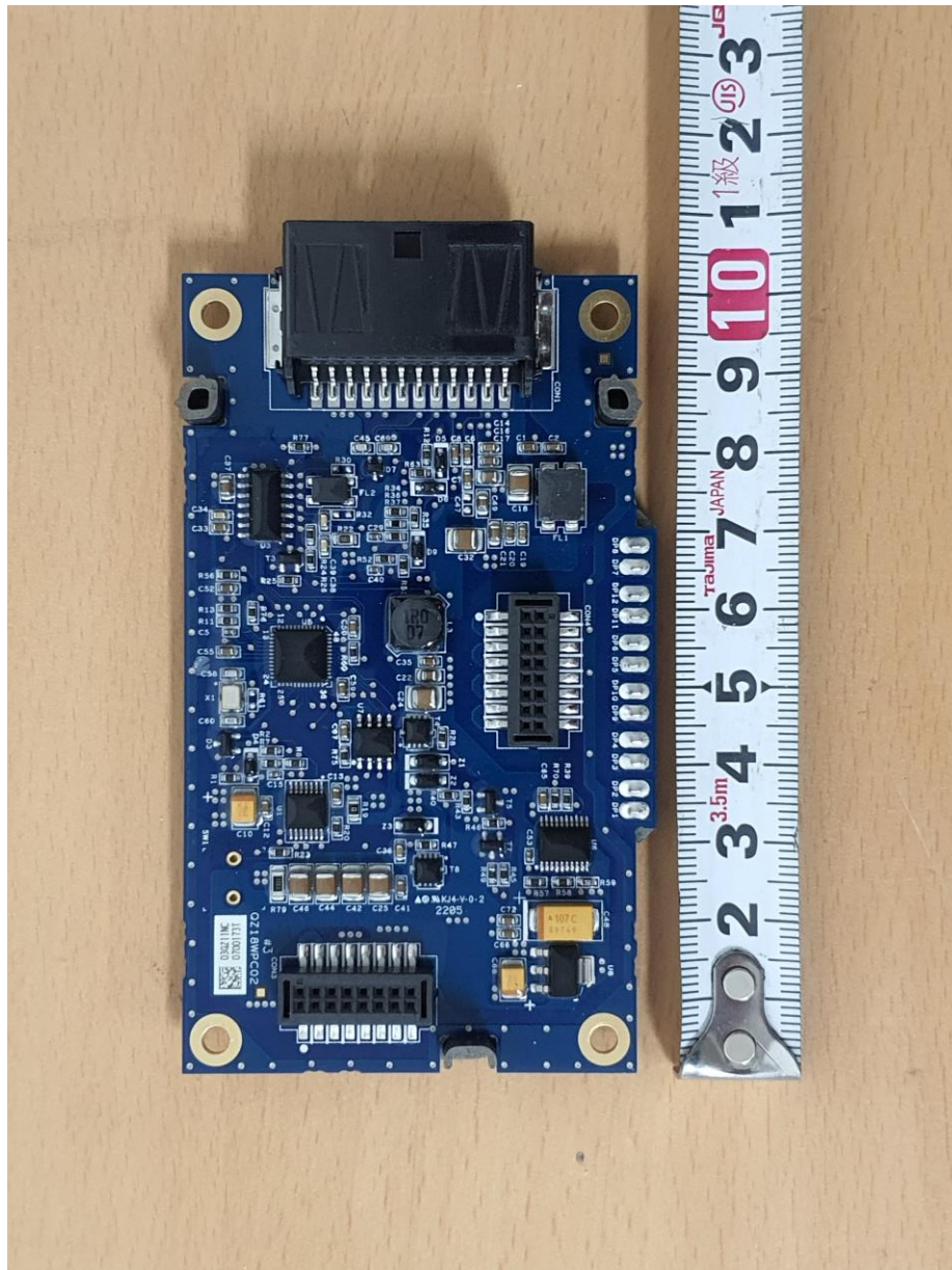
< Sub board Top view >
