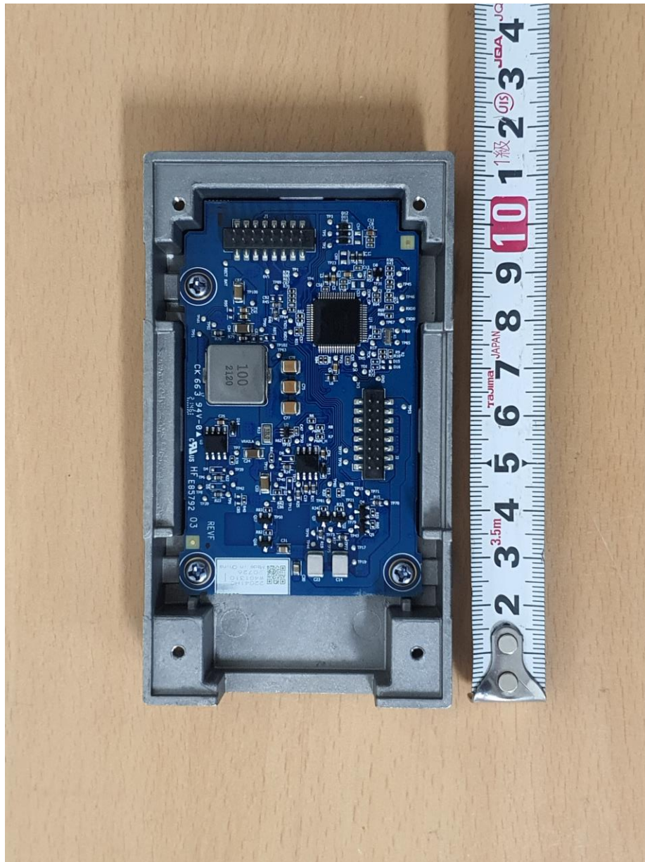
< Inside view #2 >
