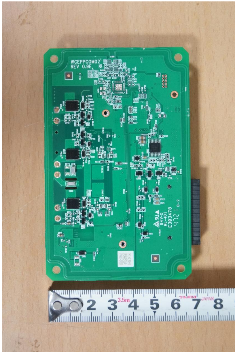
< Sub board bottom view #2 >
