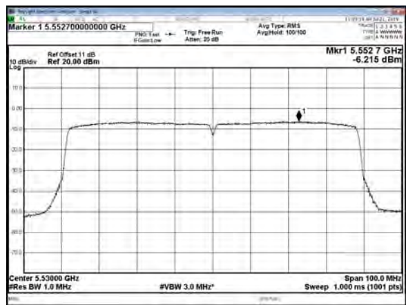
Modulation Standard: 802.11ac,VHT80 CH106
