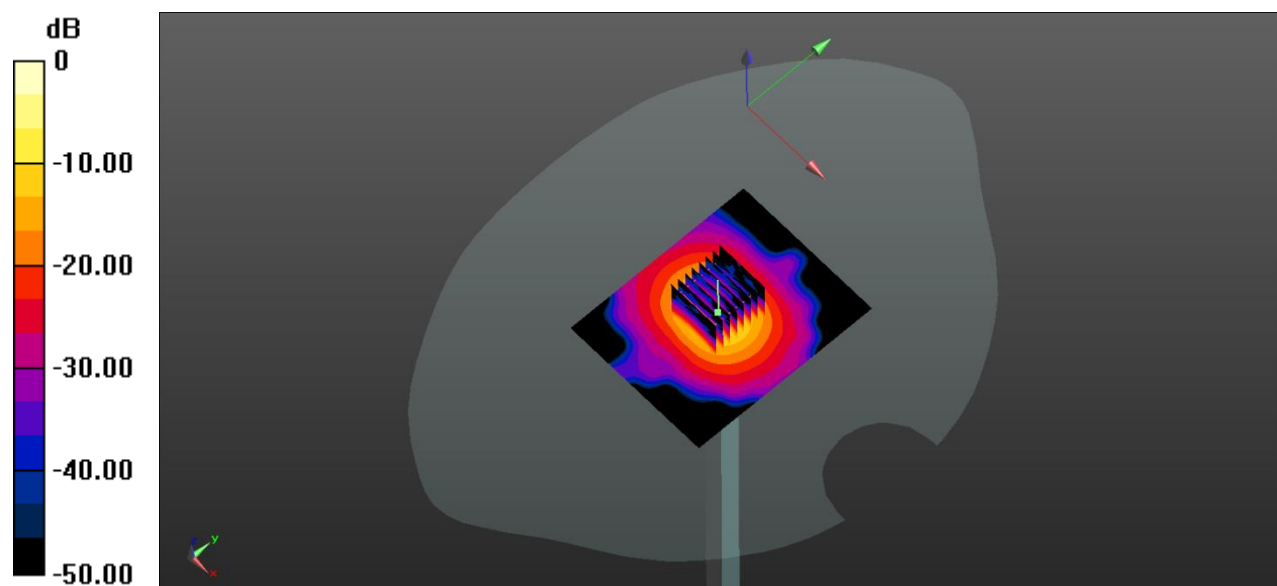
0 dB = 19.2 W/kg
