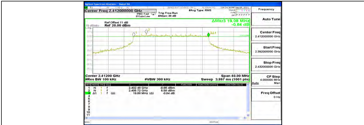
11AX20SISO Ant1 2412
