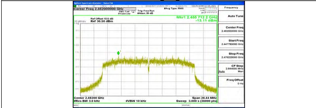
11AX20SISO Ant1 2462
