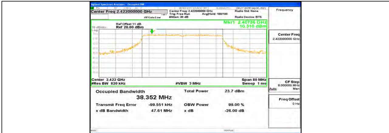
11AX40SISO Ant1 2422
