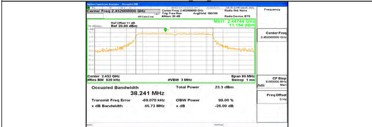
11AX40SISO Ant1 2452
