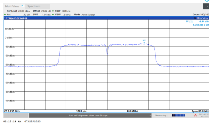
11N40SISO_Ant3_5755
