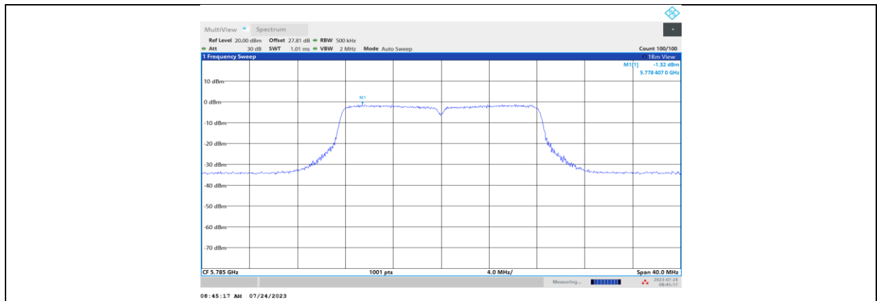
11A_Ant3_5785
