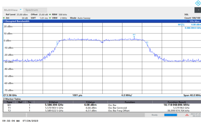
11N20SISO Ant3 5580
