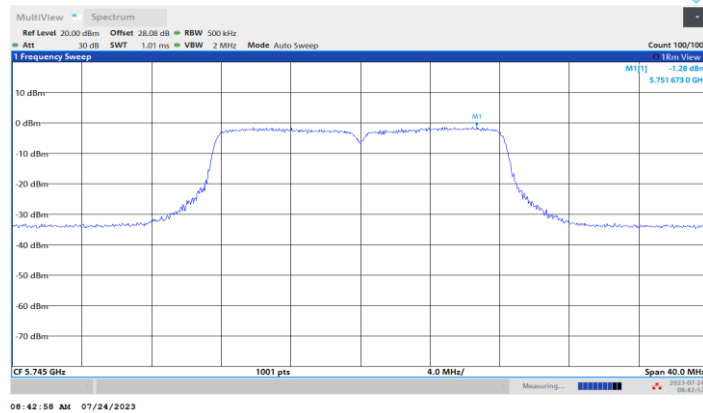
11A Ant3 5745
