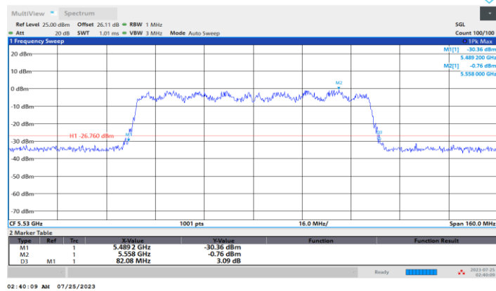
11AC80SISO_Ant3_5530
