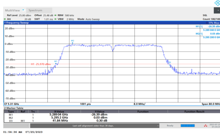
11N40SISO_Ant3_5310
