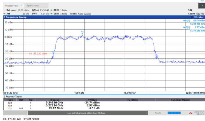
11AC80SISO_Ant3_5290
