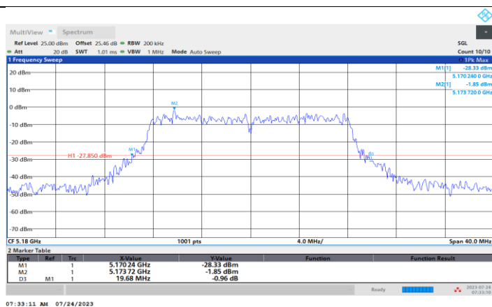
11A_Ant3_5180
