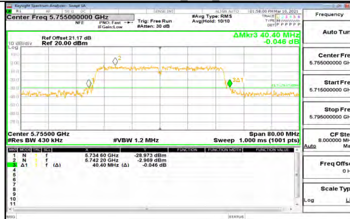
11N40SISO Ant2 5755
