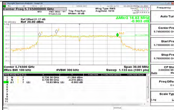
11N20SISO Ant2 5745
