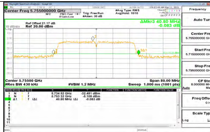
11AC40SISO Ant2 5755
