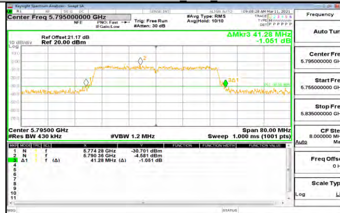
11AC40SISO Ant2 5795
