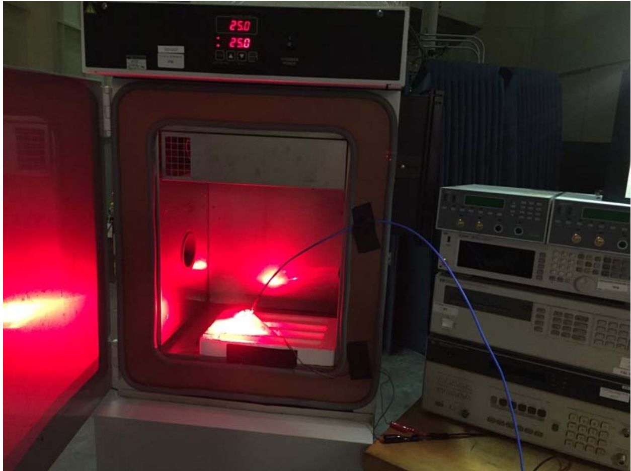
Frequency Stability 1
