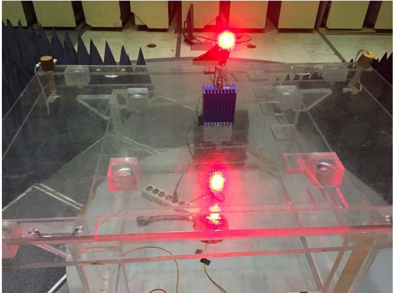
Radiated Emissions 1
