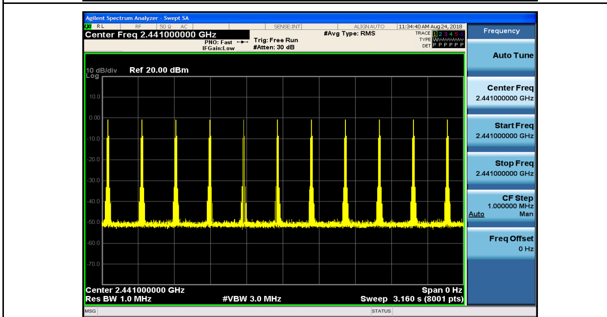
Dwell Time_2DH1_2441
