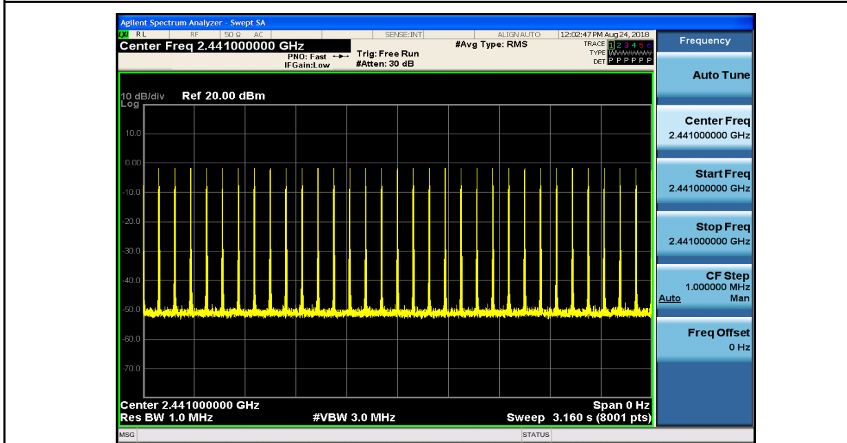
Dwell Time_3DH3_2441
