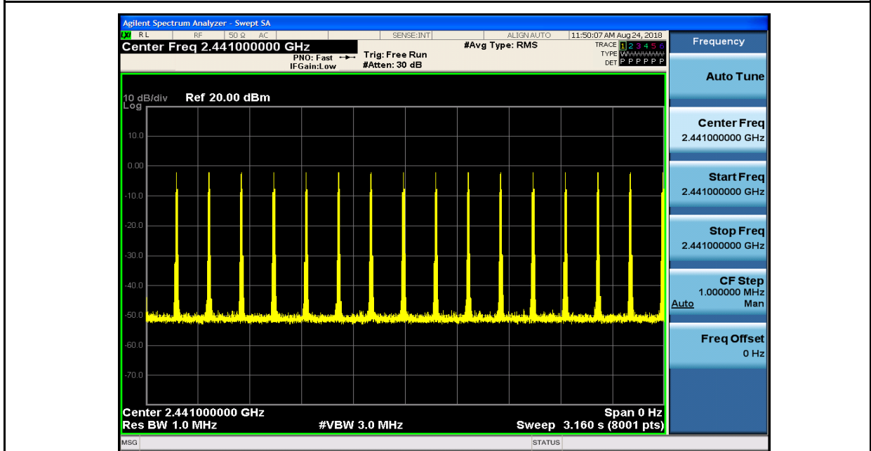
Dwell Time_3DH1_2441
