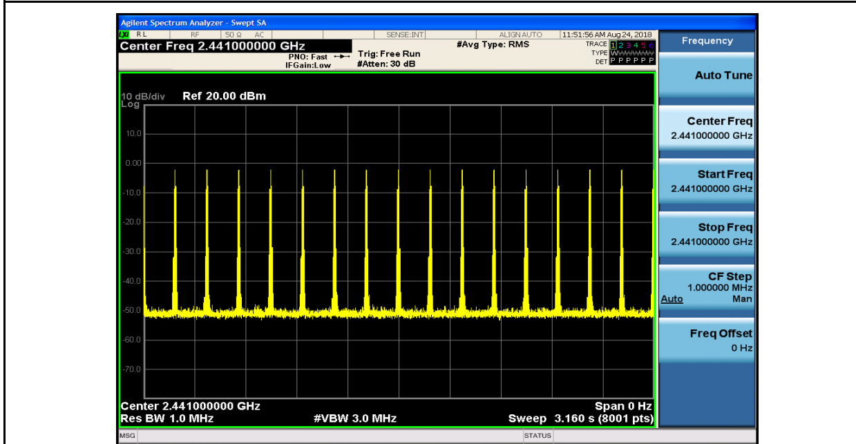
Dwell Time_2DH5_2441
