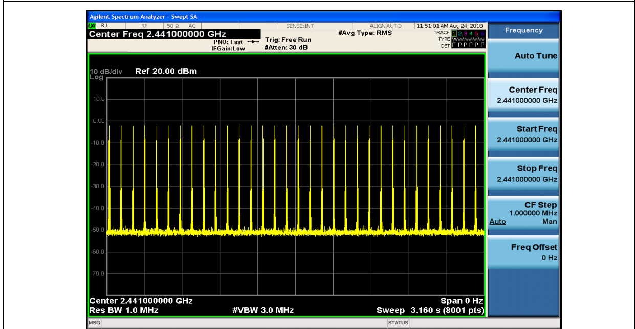
Dwell Time_2DH3_2441
