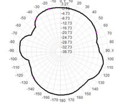
Total(H-XY), Max= 0.35dBi, CirD=10.00
