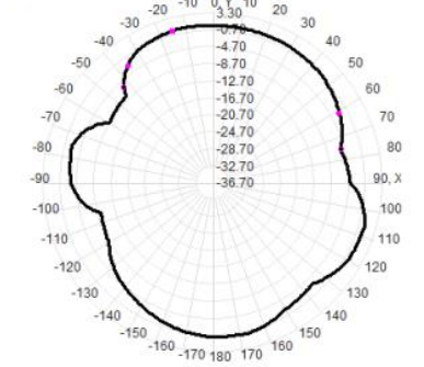
Total(H-XY), Max= 0.31dBi, CirD=9.90
