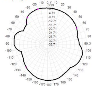
Total(H-XY), Max= 0.46dBi, CirD=10.29
