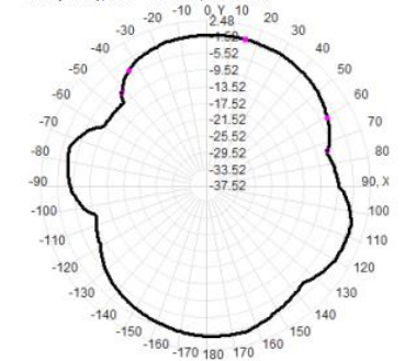
Total(H-XY), Max= -0.86dBi, CirD=9.11
