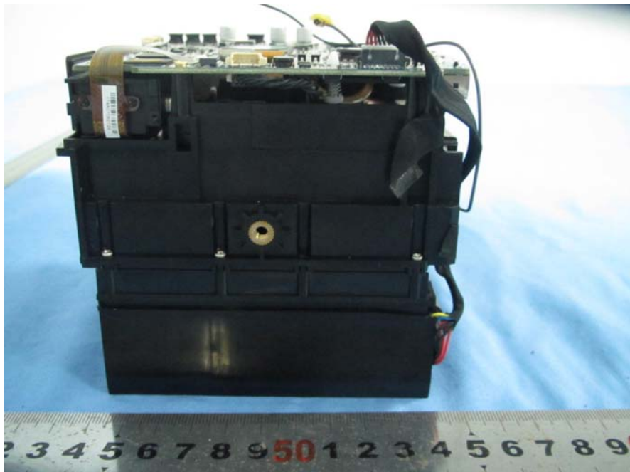
EUT_Uncovered View 4
