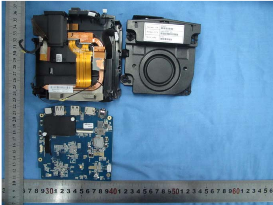
EUT_Uncovered View 7
