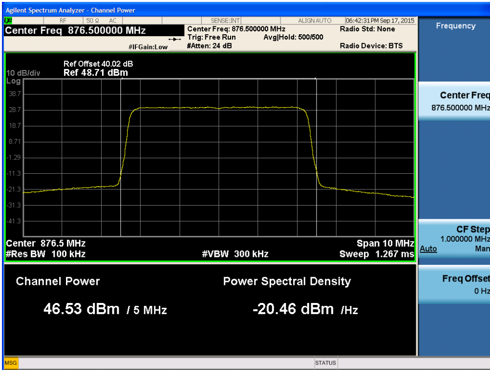
[AGC threshold Downlink LTE 5 MHz Middle]
