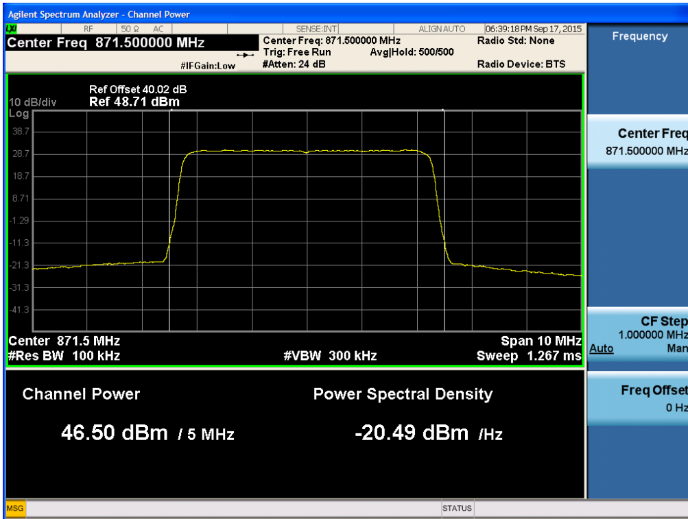
[AGC threshold Downlink LTE 5 MHz Low]
