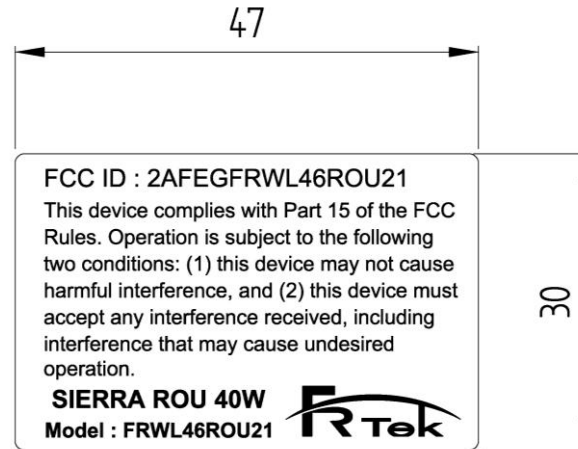
< FRWL46ROU21 label >
