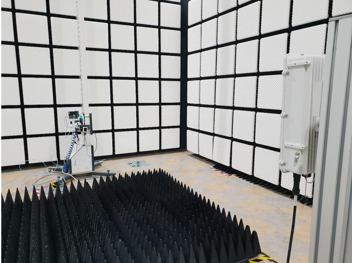
Radiated Test Setup Photo –Spurious (Horn Antenna 18 GHz ~ 40 GHz, Horizontal)
