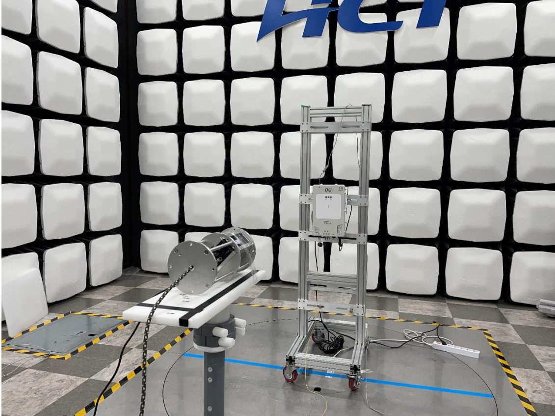
Radiated Test Setup Photo – Spurious (WR-05 Horn Antenna, 135°)
