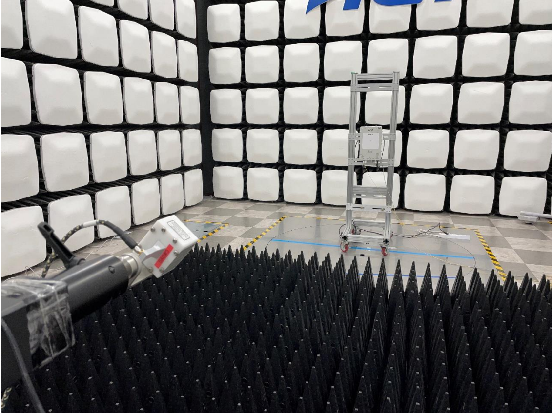
Radiated Test Setup Photo –Spurious (Horn Antenna 18 GHz ~ 40 GHz, 135°)
