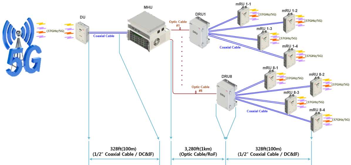
Figure 1. Network Configuration.
