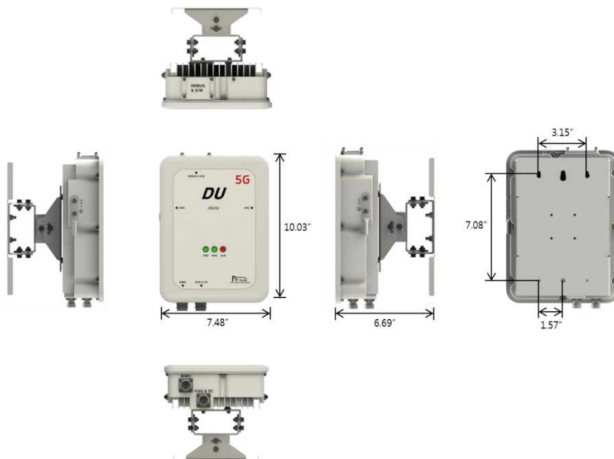
Figure 2. DU Configuration.
