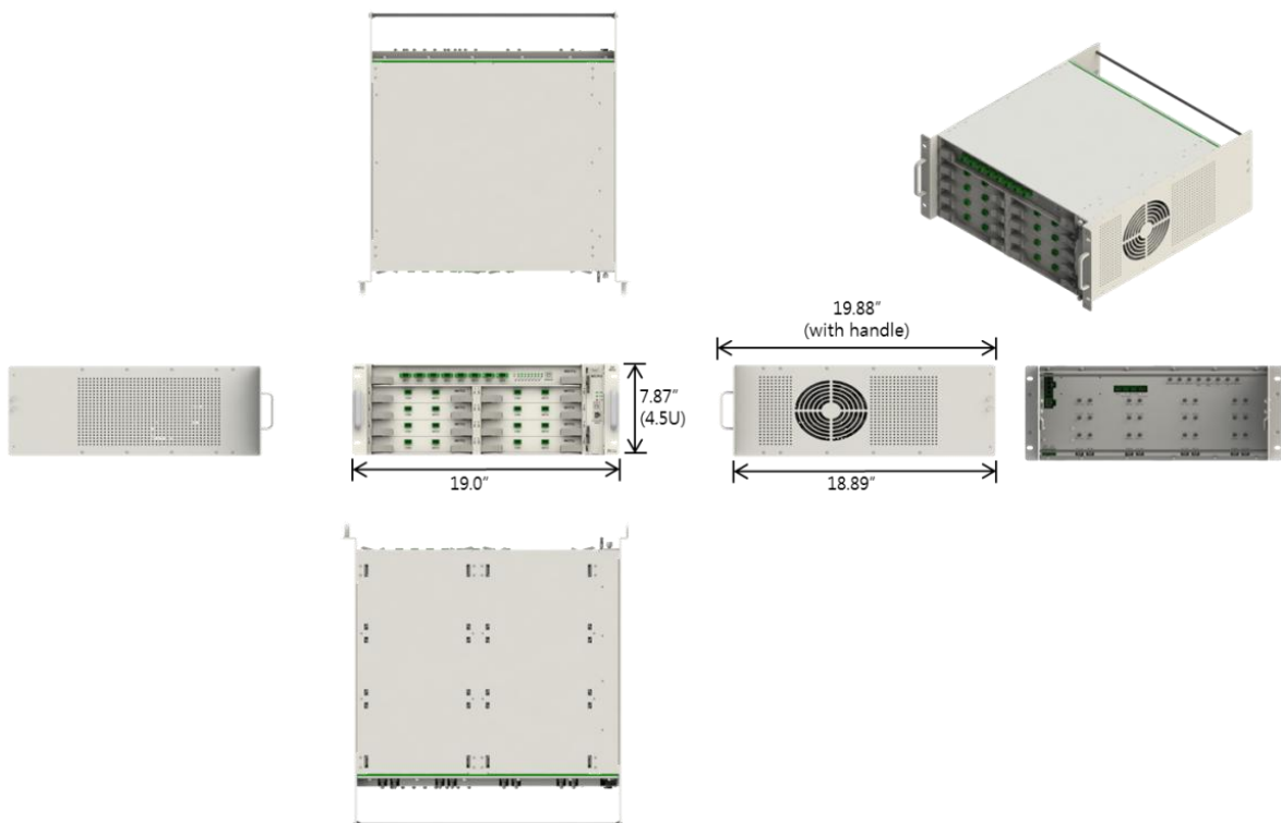
Figure 5. MHU Configuration.
