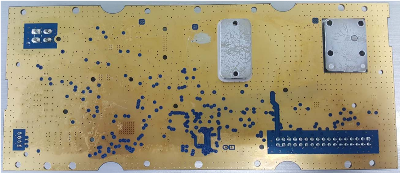
_PCB Bottom_TX
