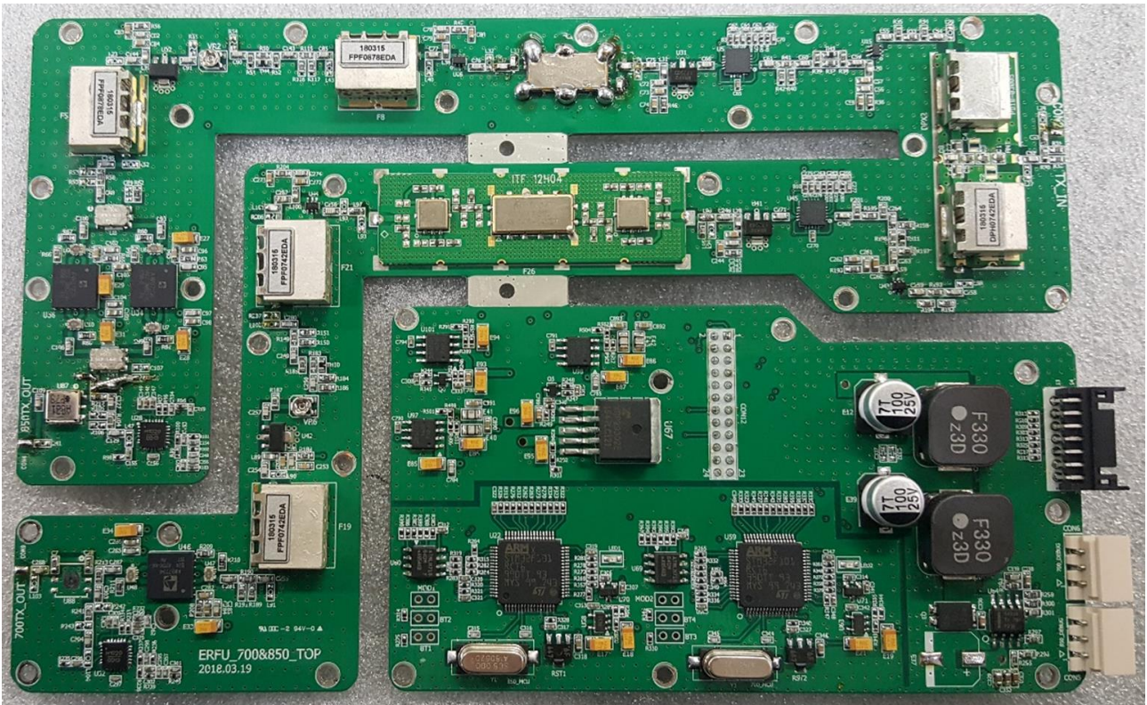
PCB_TX_Top
