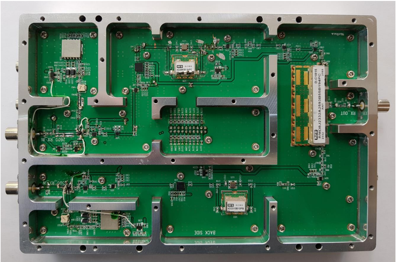
Path_Bottom
