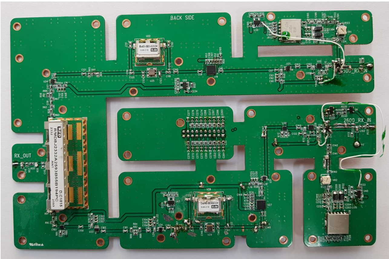
PCB_Bottom
