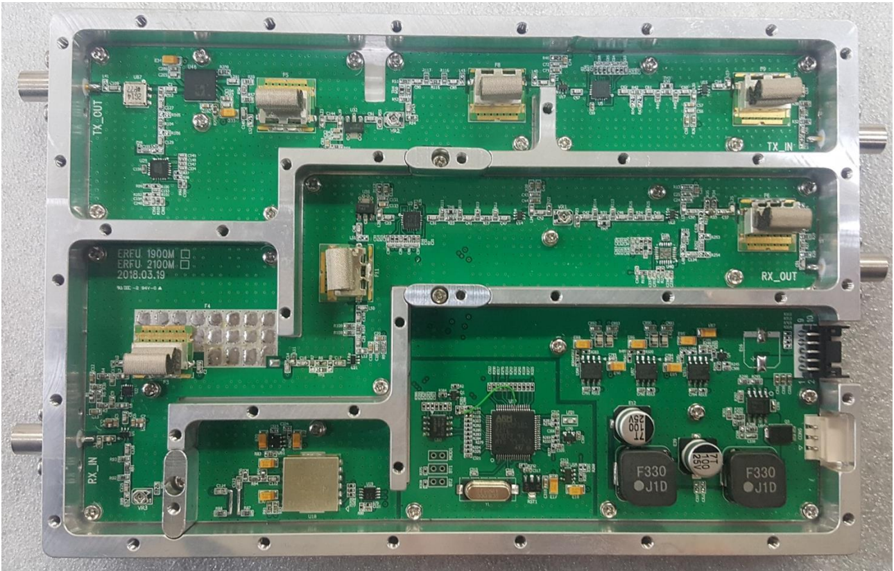
Path_Top
