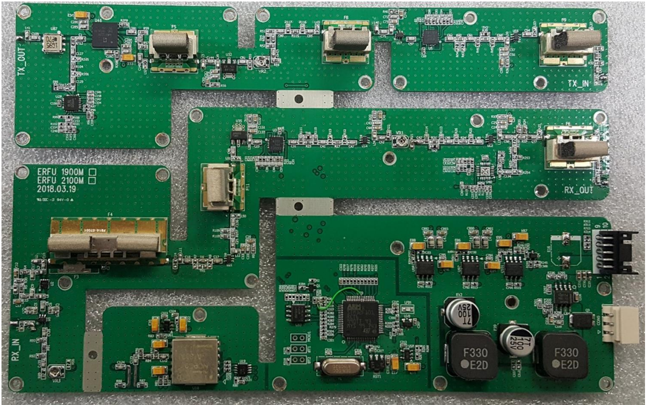
PCB_Top
