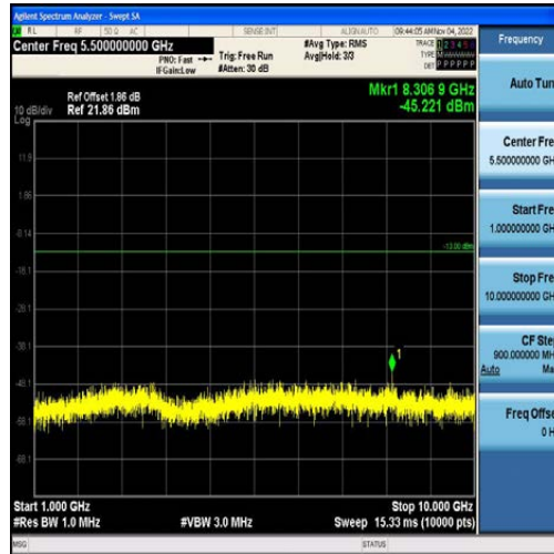
Band12-1.4MHz-QPSK-23095-6RB#0-Range2:1000~10000MHz
