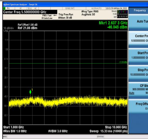
Band12-5MHz-QPSK-23155-25RB#0-Range2:1000~10000MHz
