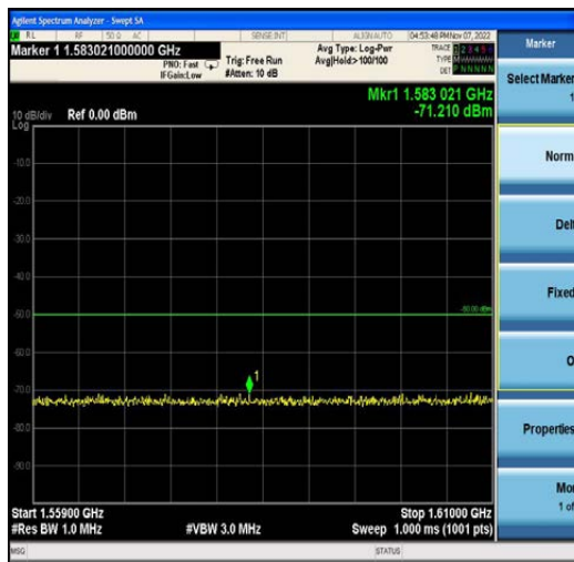
Band13-10MHz-QPSK-23230-50RB#0-Range3:1559~1610MHz
