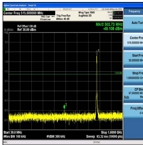
Band13-5MHz-16QAM-23205-25RB#0-Range1:30~1000MHz
