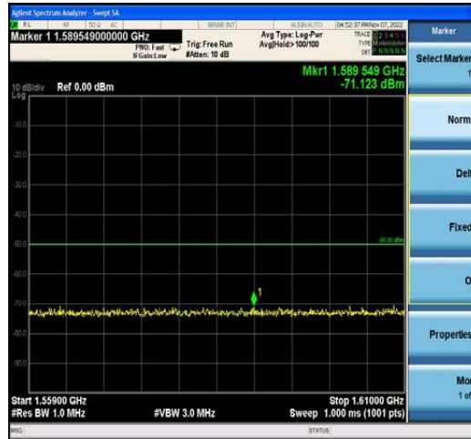
Band13-5MHz-QPSK-23230-25RB#0-Range3:1559~1610MHz
