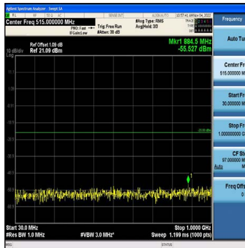
Band41-10MHz-QPSK-40620-50RB#0-Range1:30~1000MHz
