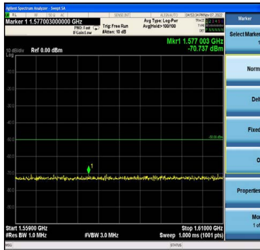
Band13-5MHz-16QAM-23255-25RB#0-Range3:1559~1610MHz
