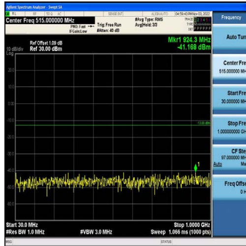
Band4-20MHz-16QAM-20300-100RB#0-Range1:30~1000MHz
