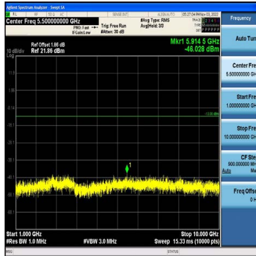
Band5-5MHz-QPSK-20525-25RB#0-Range2:1000~10000MHz
