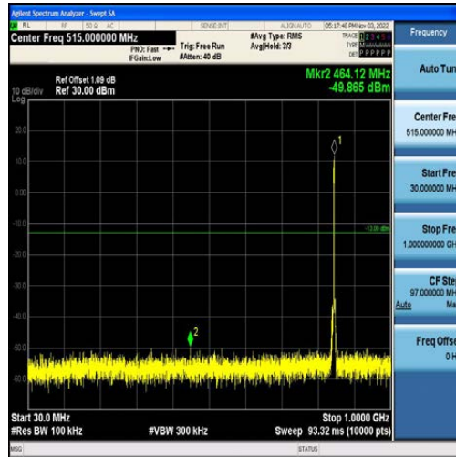
Band5-3MHz-QPSK-20635-15RB#0-Range1:30~1000MHz
