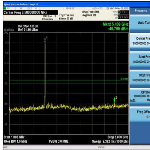
Band7-15MHz-QPSK-20825-75RB#0-Range2:1000~6000MHz
