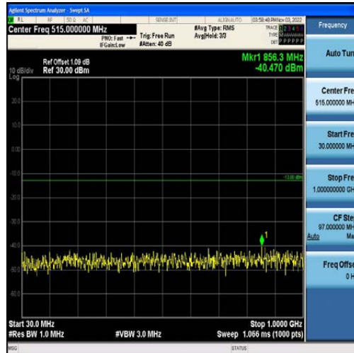
Band2-15MHz-16QAM-18675-75RB#0-Range1:30~1000MHz
