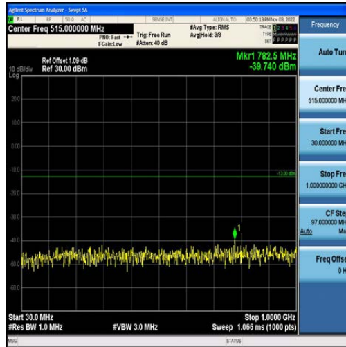
Band2-10MHz-16QAM-18650-50RB#0-Range1:30~1000MHz
