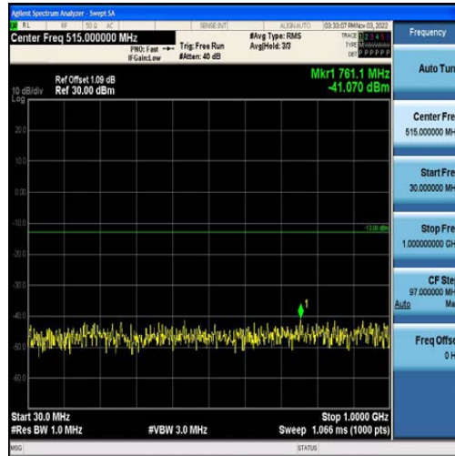
Band2-3MHz-16QAM-18615-15RB#0-Range1:30~1000MHz
