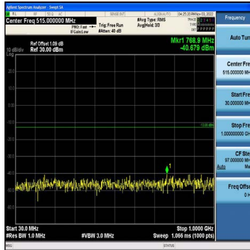
Band4-3MHz-16QAM-20385-15RB#0-Range1:30~1000MHz
