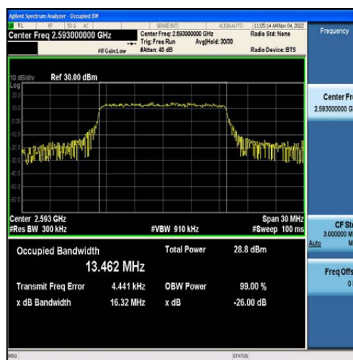
Band41-15MHz-QPSK-40620-75RB#0-13.462
