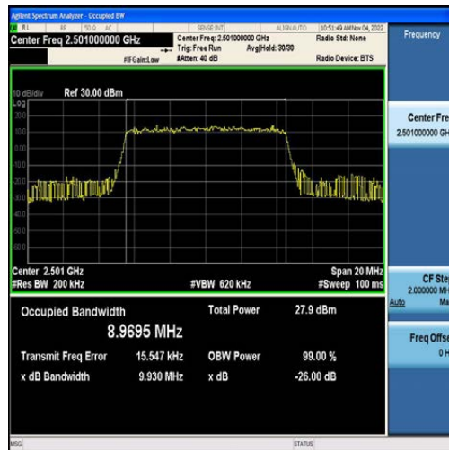
Band41-10MHz-16QAM-39700-50RB#0-8.9695
