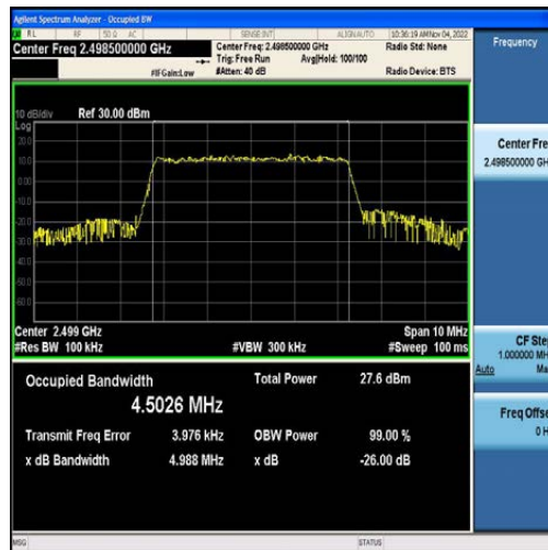
Band41-5MHz-16QAM-39675-25RB#0-4.5026
