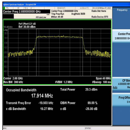
Band41-20MHz-QPSK-41490-100RB#0-17.914
