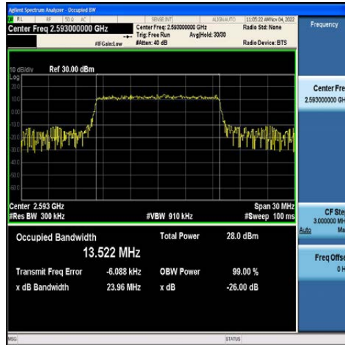
Band41-15MHz-16QAM-40620-75RB#0-13.522
