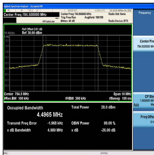
Band13-5MHz-QPSK-23255-25RB#0-4.4965
