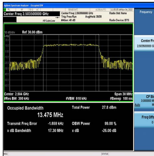
Band41-15MHz-16QAM-39725-75RB#0-13.475
