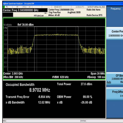
Band41-10MHz-16QAM-40620-50RB#0-8.9702
