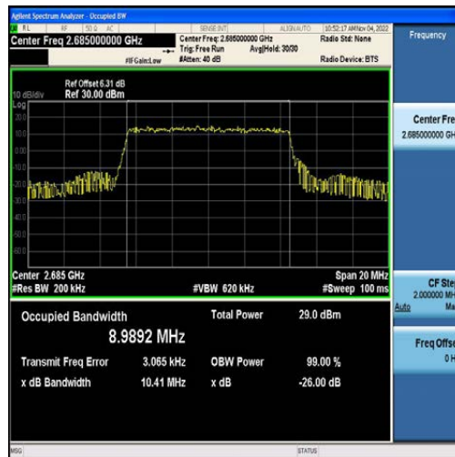
Band41-10MHz-QPSK-41540-50RB#0-8.9892
