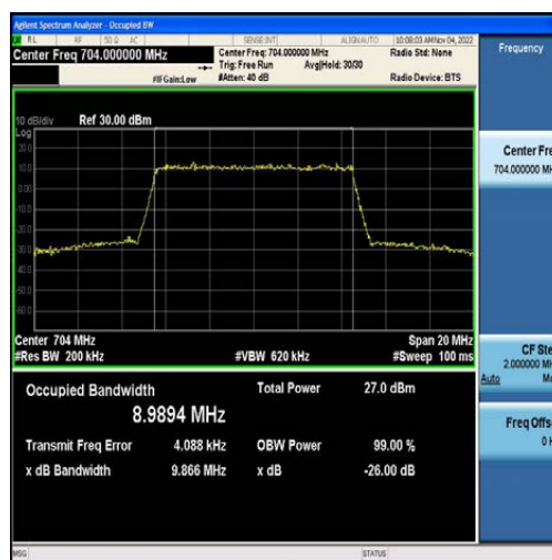
Band12-10MHz-16QAM-23060-50RB#0-8.9894
