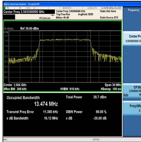
Band41-15MHz-QPSK-39725-75RB#0-13.474
