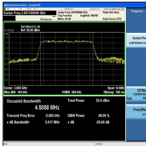
Band41-5MHz-QPSK-41565-25RB#0-4.5058
