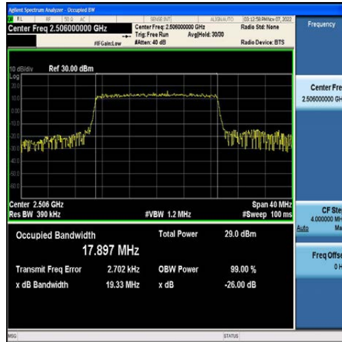
Band41-20MHz-QPSK-39750-100RB#0-17.897
