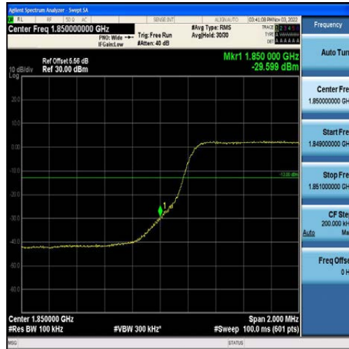
Band2-5MHz-16QAM-18625-25RB#0
