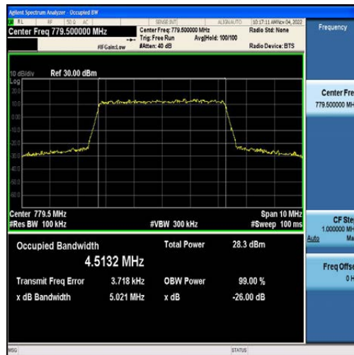
Band13-5MHz-QPSK-23205-25RB#0-4.5132
