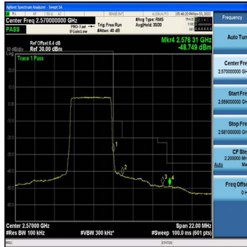
Band7-5MHz-QPSK-21425-25RB#0
