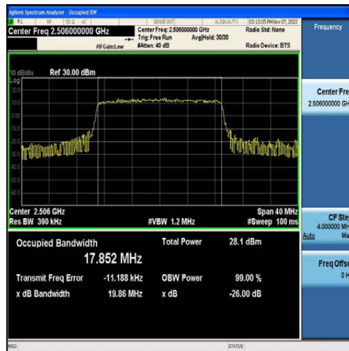
Band41-20MHz-16QAM-39750-100RB#0-17.852
