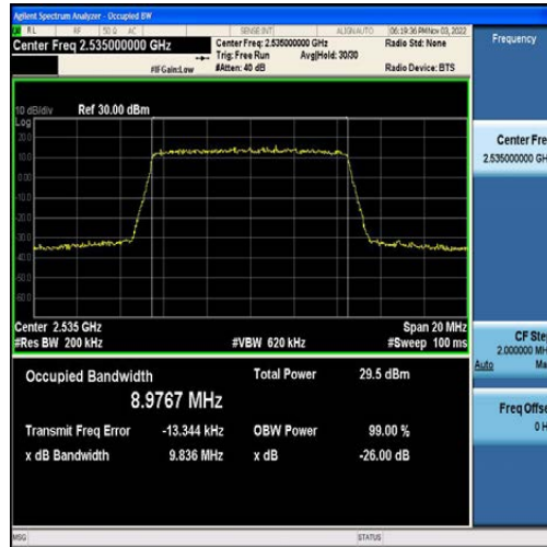
Band7-10MHz-QPSK-21100-50RB#0-8.9767
