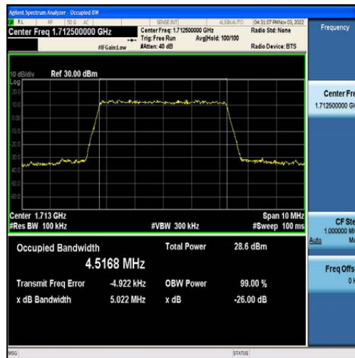
Band4-5MHz-QPSK-19975-25RB#0-4.5168
