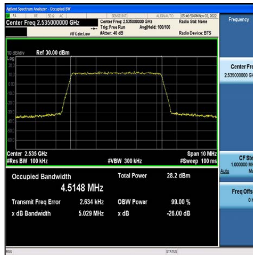
Band7-5MHz-16QAM-21100-25RB#0-4.5148
