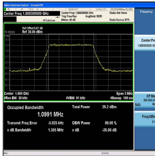
Band2-1.4MHz-16QAM-19193-6RB#0-1.0991
