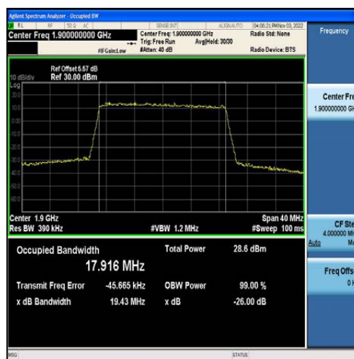
Band2-20MHz-QPSK-19100-100RB#0-17.916
