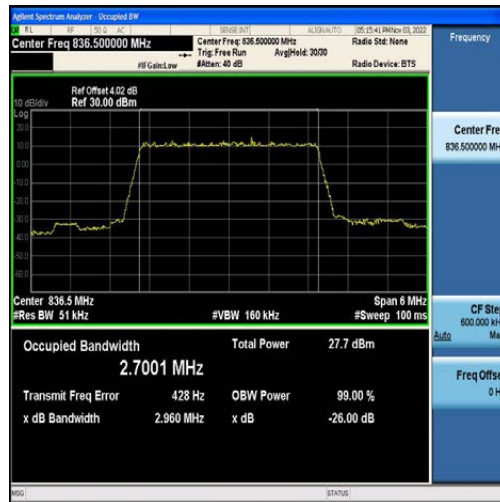
Band5-3MHz-QPSK-20525-15RB#0-2.7001
