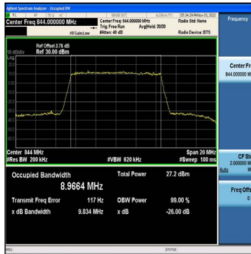
Band5-10MHz-16QAM-20600-50RB#0-8.9664
