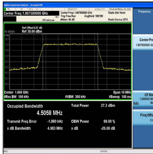
Band2-5MHz-16QAM-19175-25RB#0-4.5058
