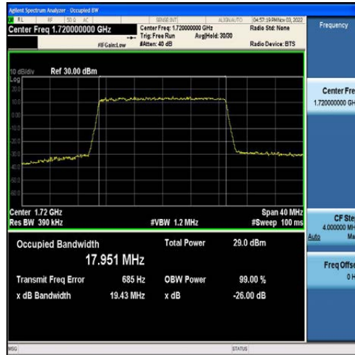
Band4-20MHz-QPSK-20050-100RB#0-17.951
