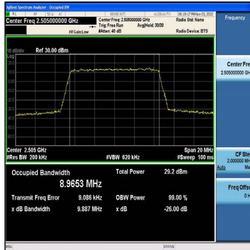
Band7-10MHz-QPSK-20800-50RB#0-8.9653
