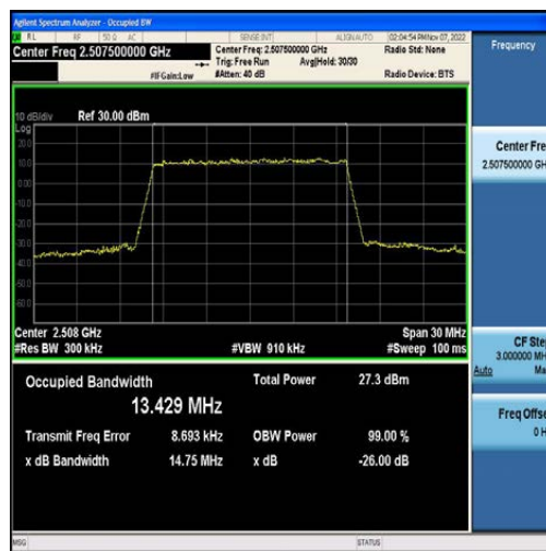
Band7-15MHz-16QAM-20825-75RB#0-13.429
