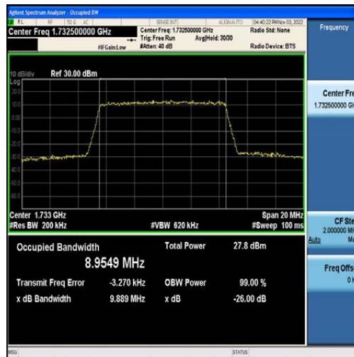
Band4-10MHz-16QAM-20175-50RB#0-8.9549
