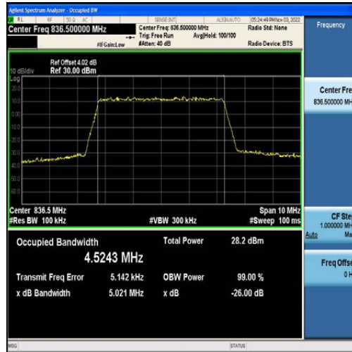
Band5-5MHz-QPSK-20525-25RB#0-4.5243
