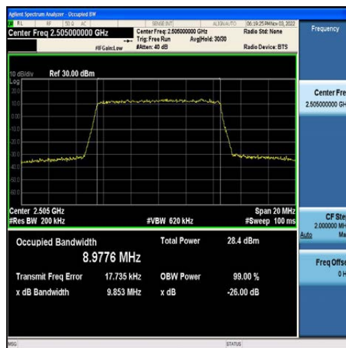
Band7-10MHz-16QAM-20800-50RB#0-8.9776
