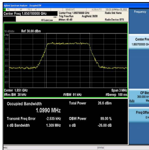
Band2-1.4MHz-16QAM-18607-6RB#0-1.0990
