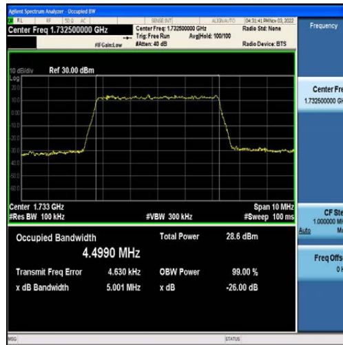
Band4-5MHz-QPSK-20175-25RB#0-4.4990
