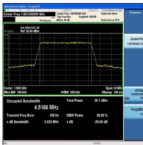
Band2-5MHz-QPSK-19175-25RB#0-4.5166
