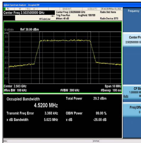
Band7-5MHz-QPSK-20775-25RB#0-4.5200
