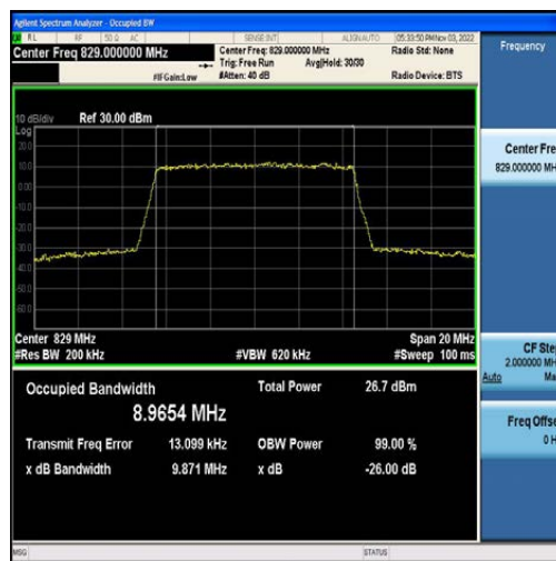
Band5-10MHz-16QAM-20450-50RB#0-8.9654
