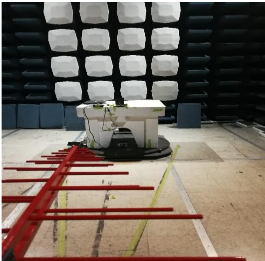
Figure R4: Radiated Emissions 30M-1G Test Setup
