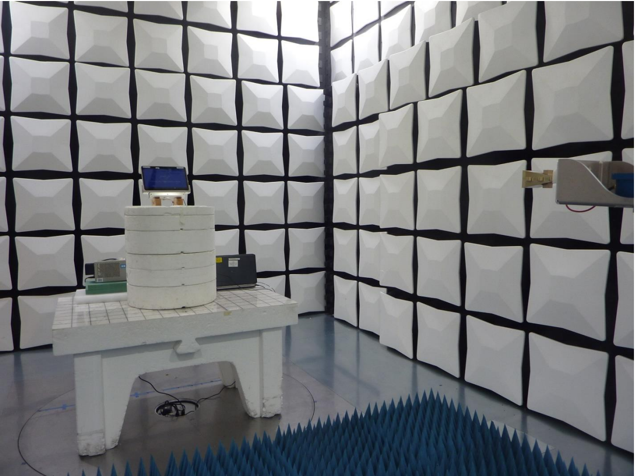
Figure 5: Test Setup for Radiated Emissions 18GHz to 40 GHz- Front View
