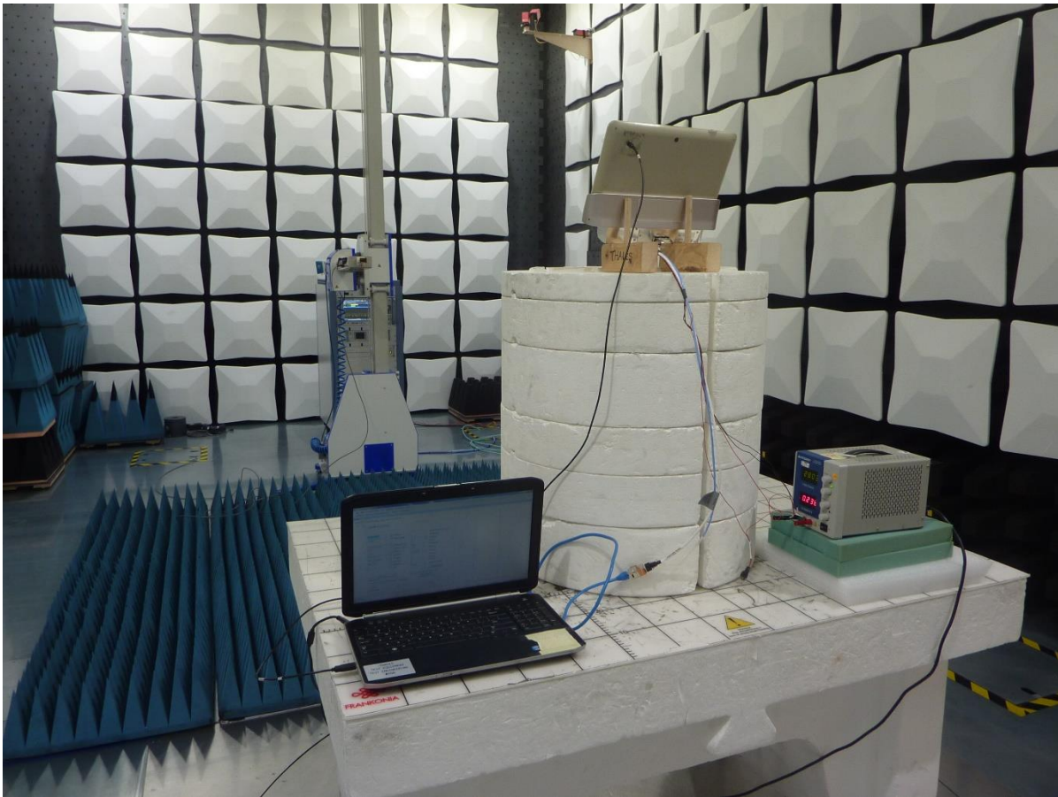
Figure 6: Test Setup for Radiated Emissions 18GHz to 40 GHz -Rear View
