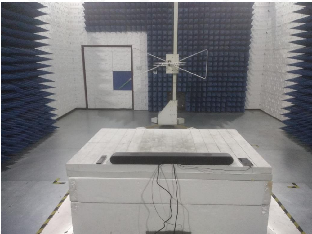
RADIATED EMISSION TEST SETUP BELOW 1GHZ-BACK
