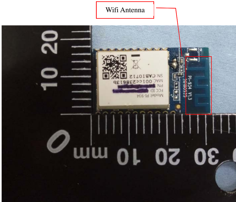
EUT View 1
