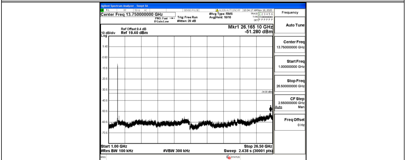
11N20SISO_Ant1_2437_0~Reference
