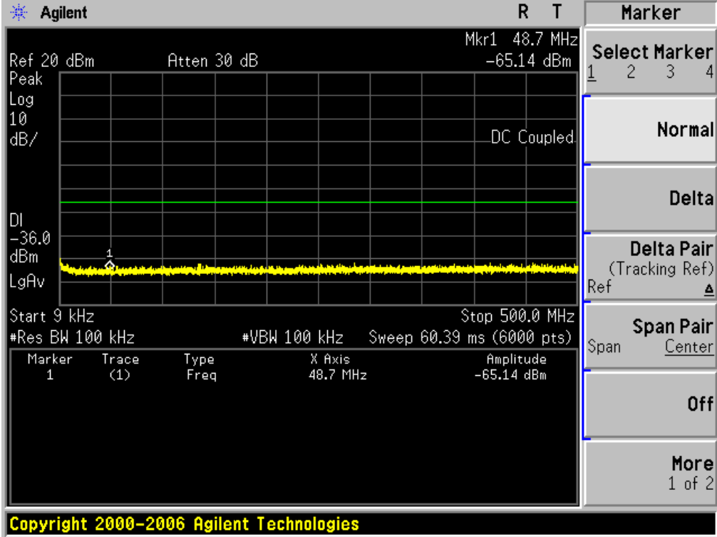
TEST PLOT OF OUT OF BAND EMISSIONS WITH THE WORST CASE OF GFSK MODULATION IN LOW CHANNEL
