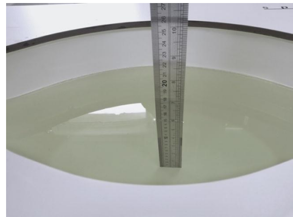
Liquid depth in the body phantom (2450MHz)
