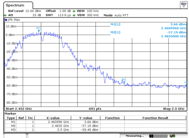
CH11-Bandedge
