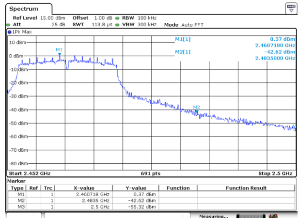
CH11-Bandedge
