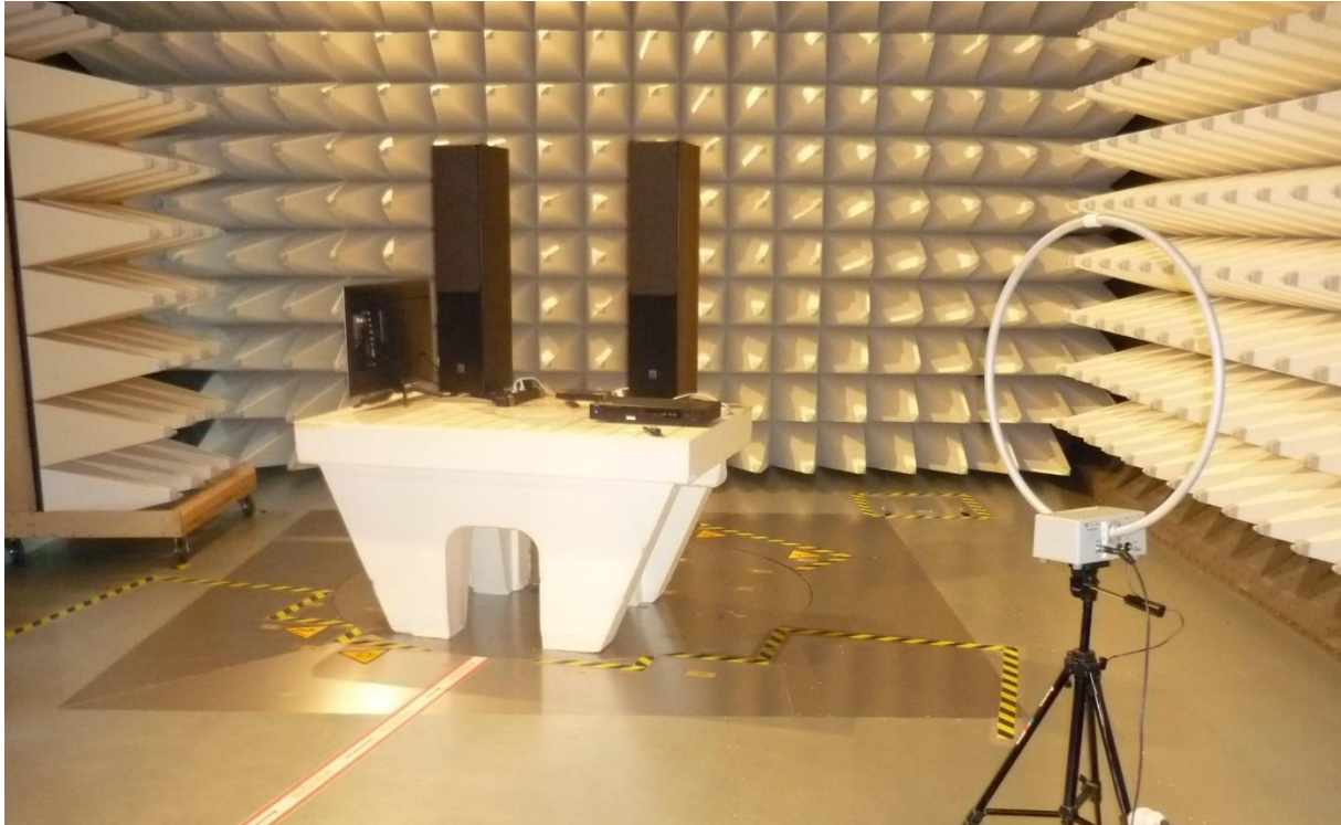
Tested frequency range 9 kHz – 30 MHz
