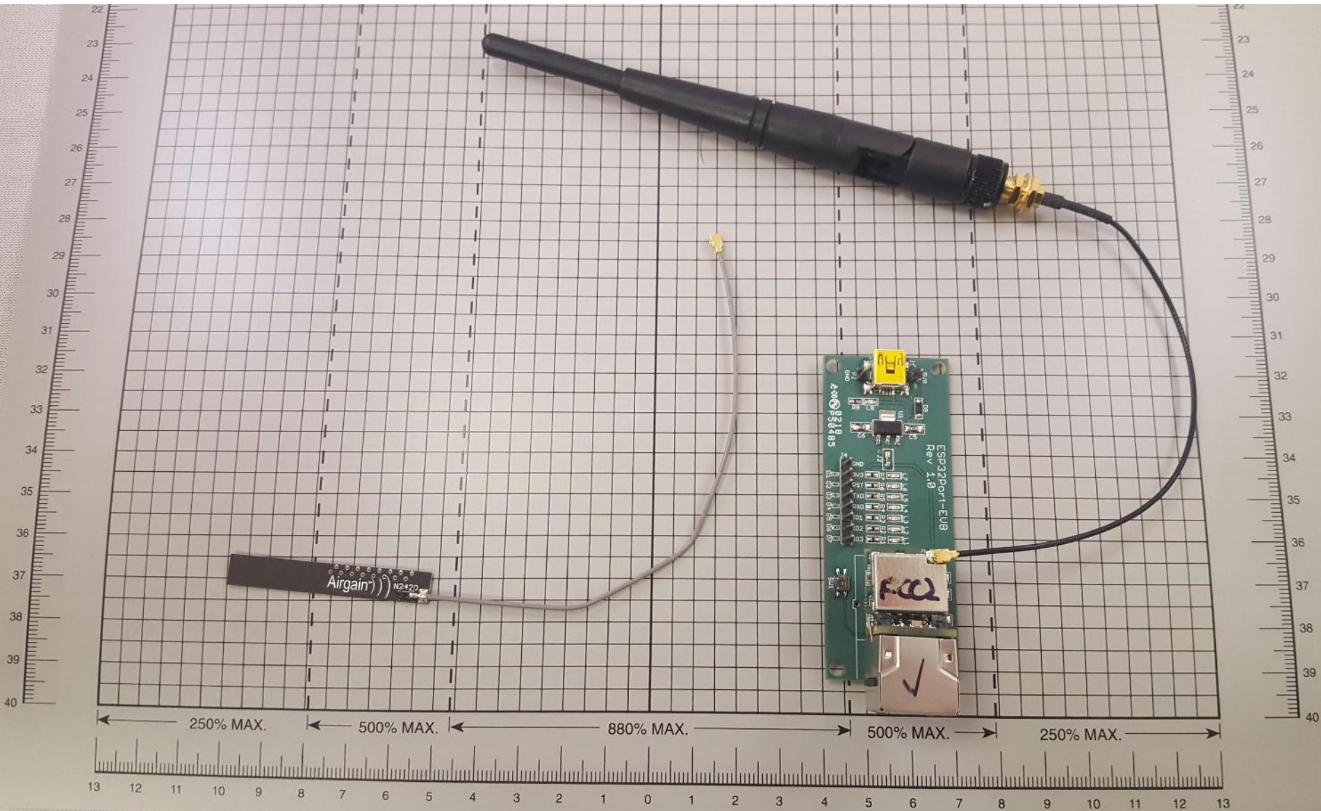
EUT mounted on Interface Board with Whip and PCB Antennas
