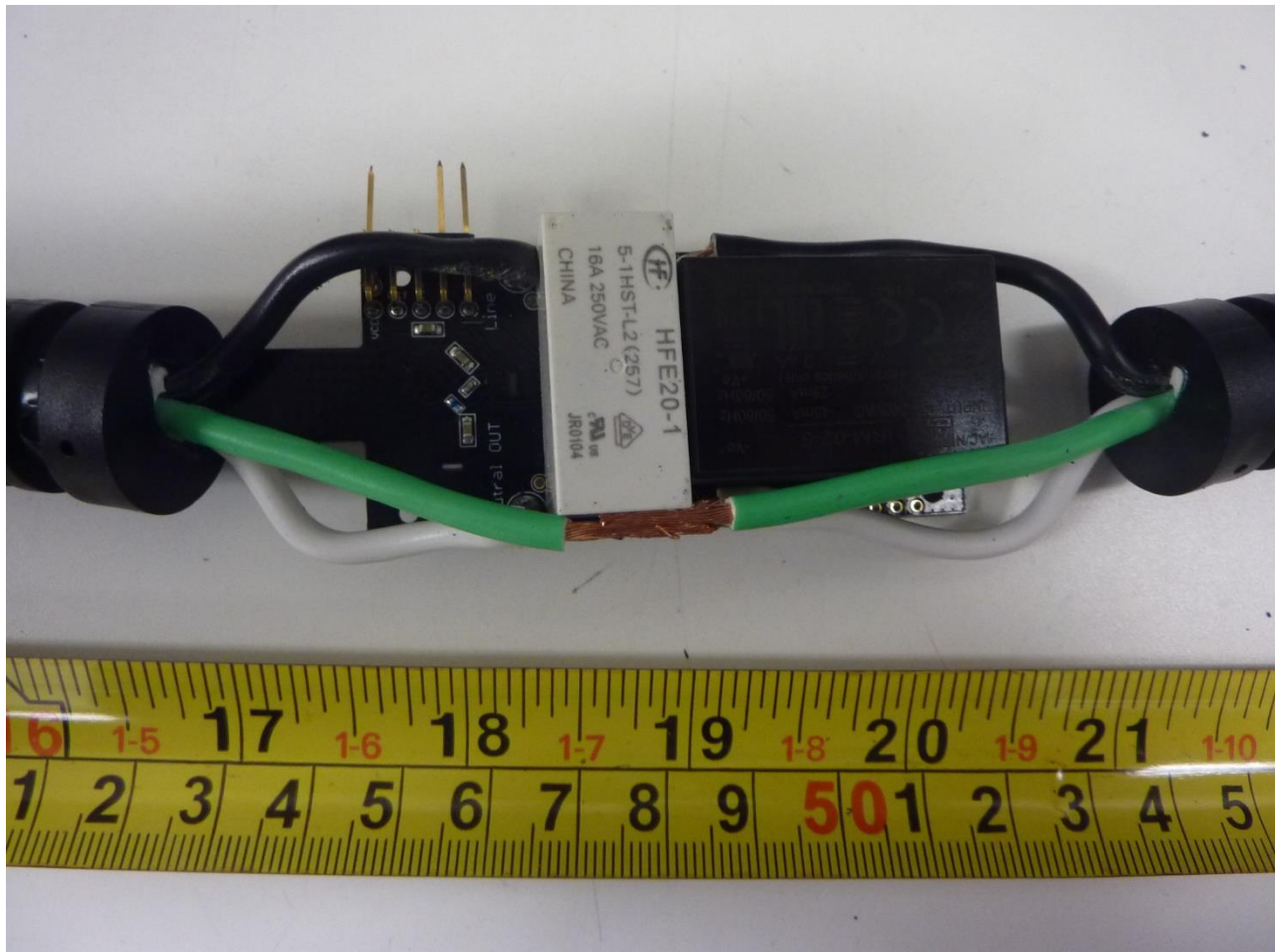
Figure 2 - Internal Photo of EUT- Top View
