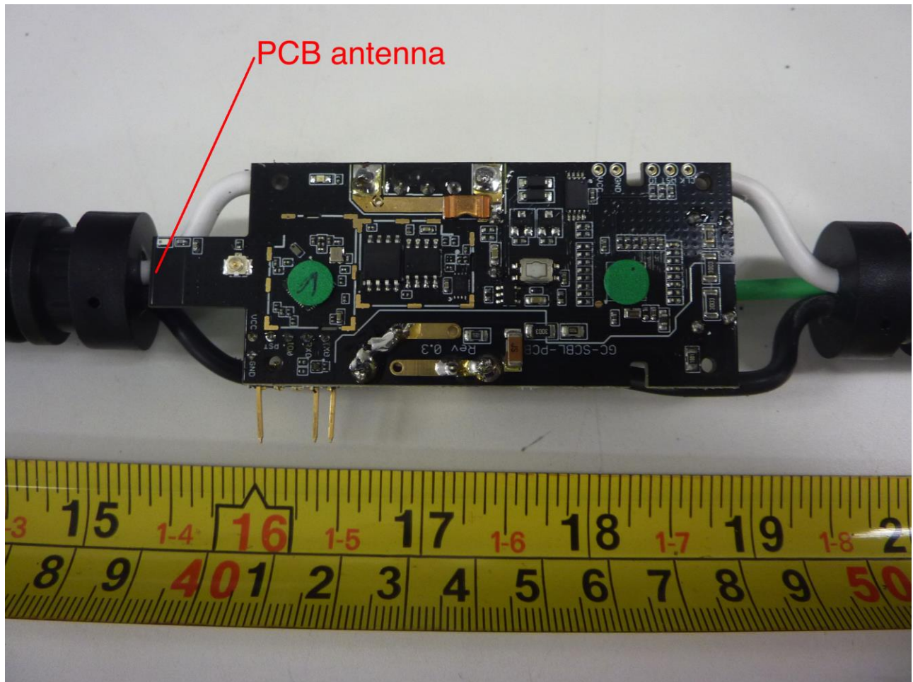
Figure 4 - Internal Photo of EUT- Antenna Location View
