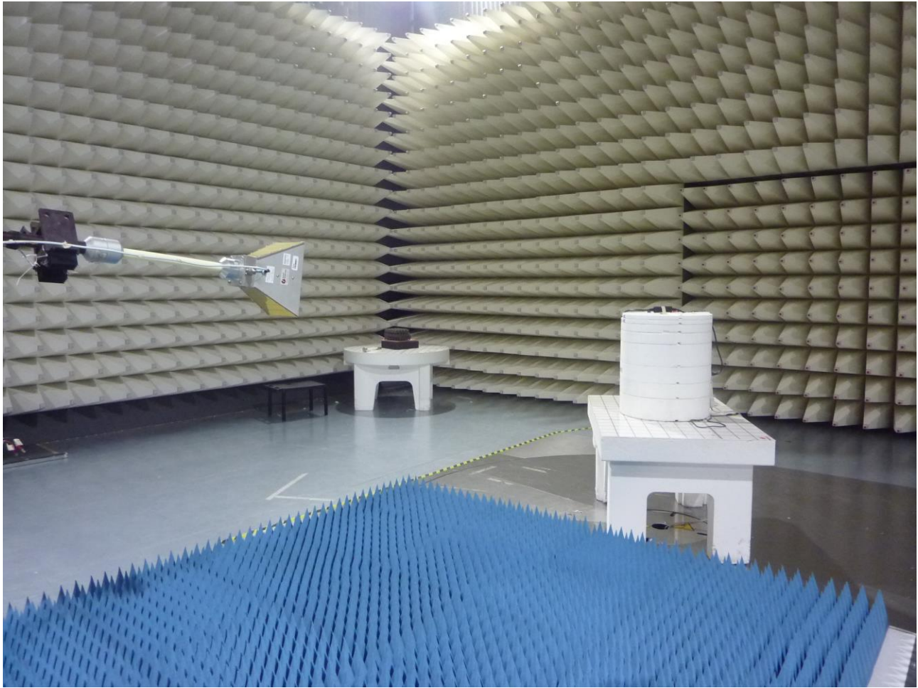
Figure 4: Test Setup for Radiated Emissions 1GHz to 18GHz (WIFI and BT LE Modes)
