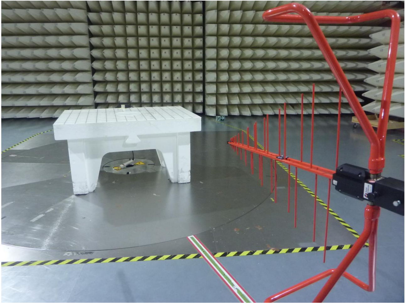
Figure 3: Test Setup for Radiated Emissions 30MHz to 1000MHz (WIFI, BT LE, and Unintentional Modes)
