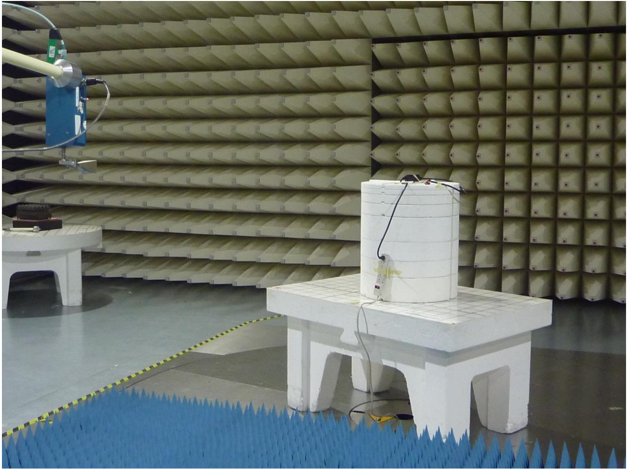
Figure 5: Test Setup for Radiated Emissions 18GHz to 26 GHz (WIFI and BT LE Modes)
