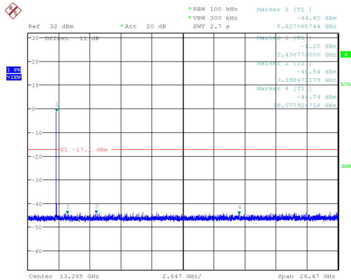
Plot 53. 802.11b CCK, 2437MHz, 30MHz-26.5GHz Non-restricted Out of Band
