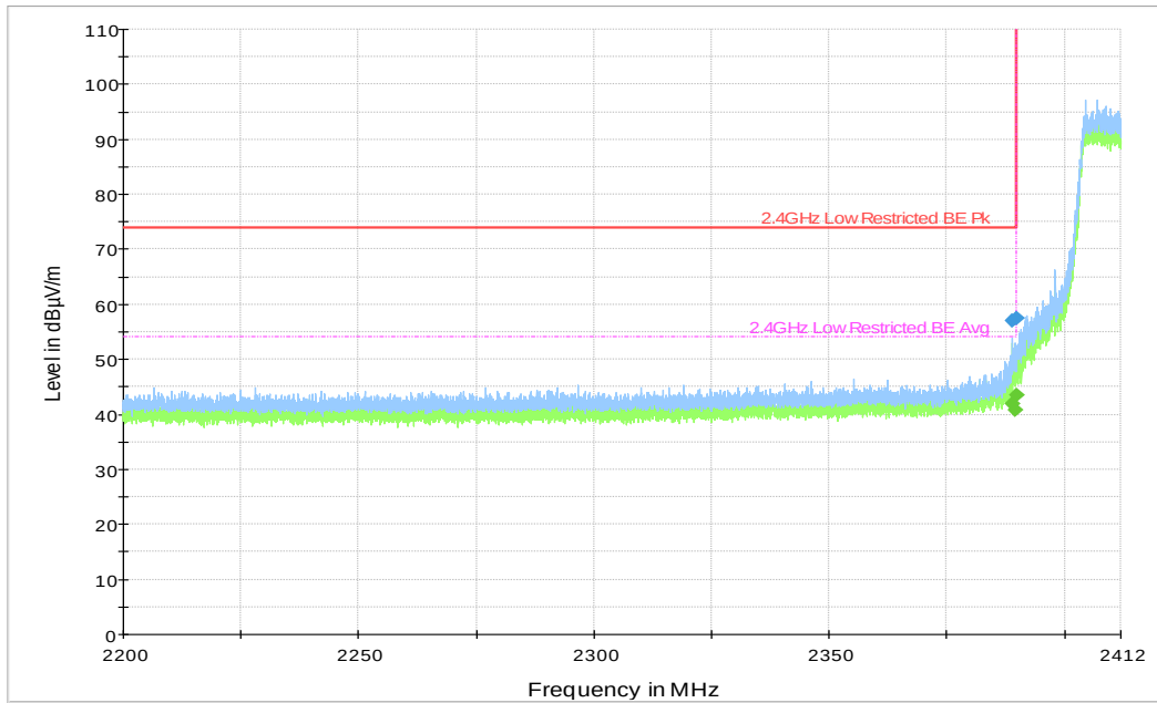
Plot 77. 802.11n HT20, 2412MHz, Lower Band Edge, Restricted
