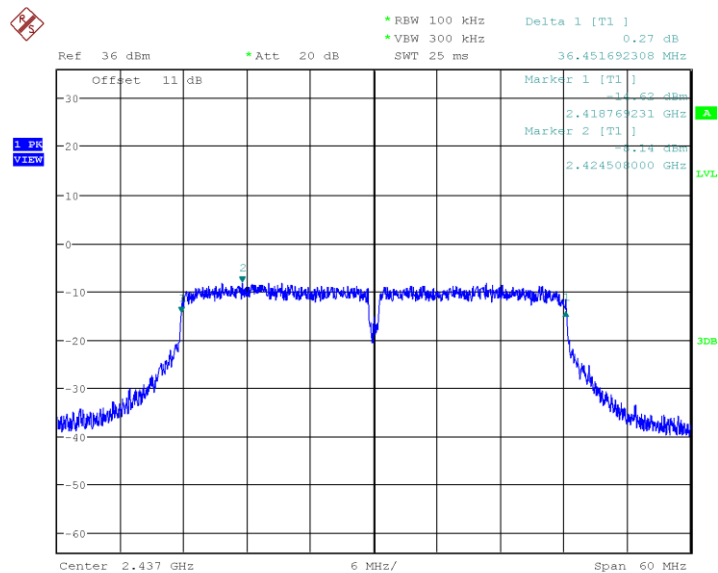
Plot 9. 802.11n(HT40), 2437MHz, 6dB Bandwidth
