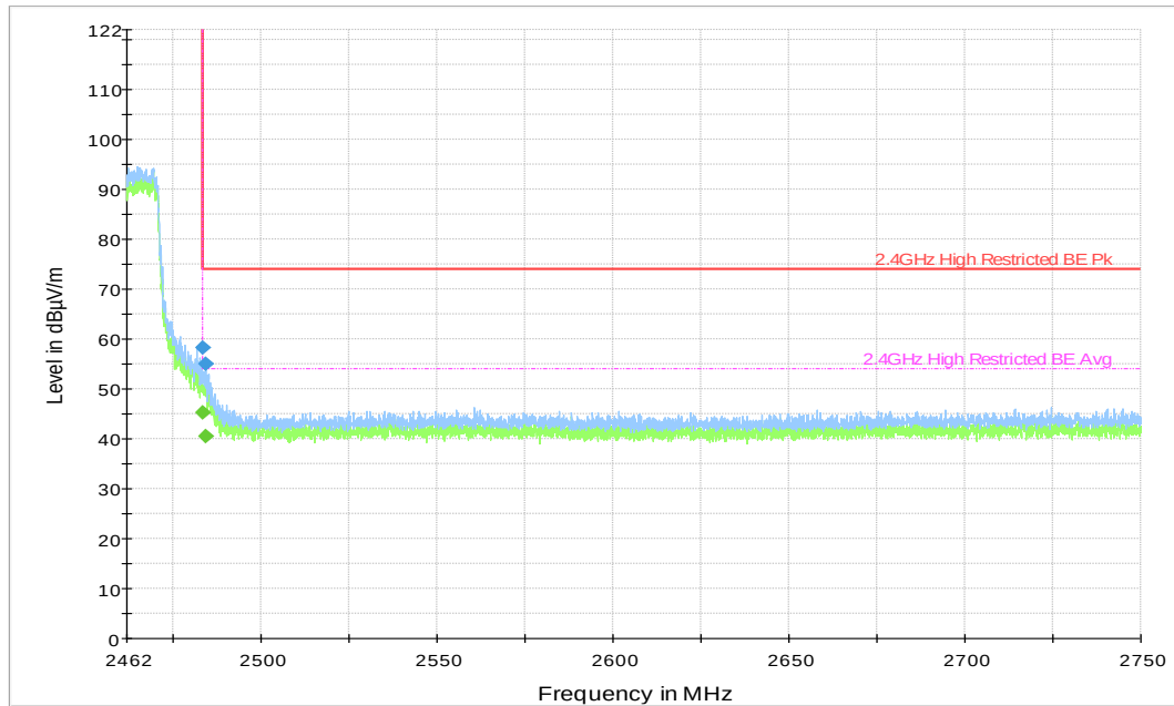
Plot 81. 802.11n HT20, 2462MHz, Upper Band Edge, Restricted
