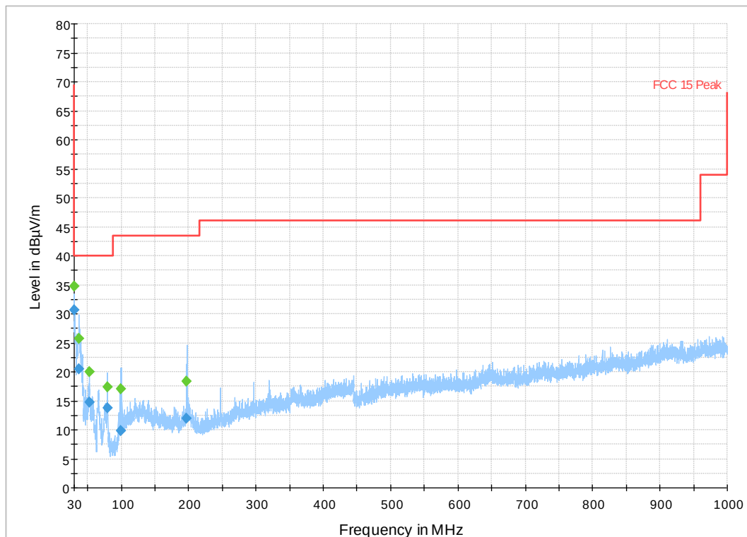
Plot 83. 30MHz-1GHz 802.11b Mode, Channel 11
