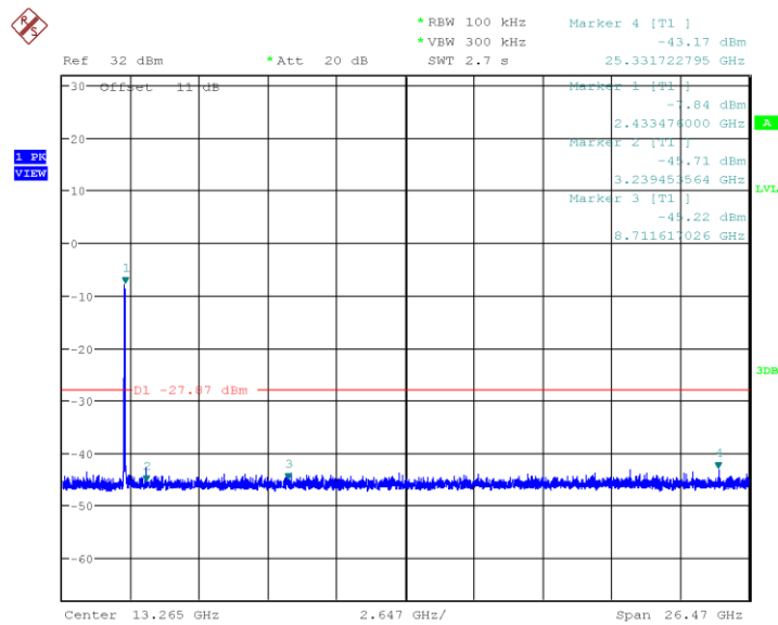
Plot 73. 802.11n HT40, 2452MHz, 30MHz-26.5GHz Non-restricted Out of Band
