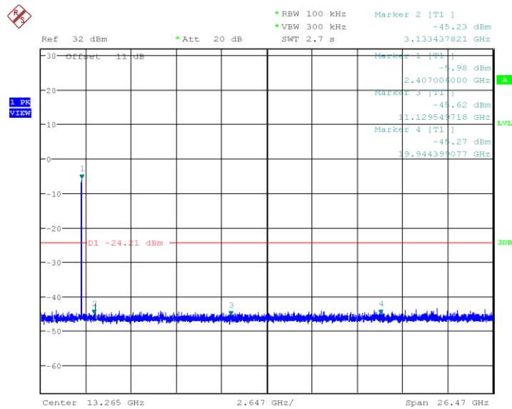
Plot 63. 802.11n HT20, 2412MHz, 30MHz-26.5GHz Non-restricted Out of Band
