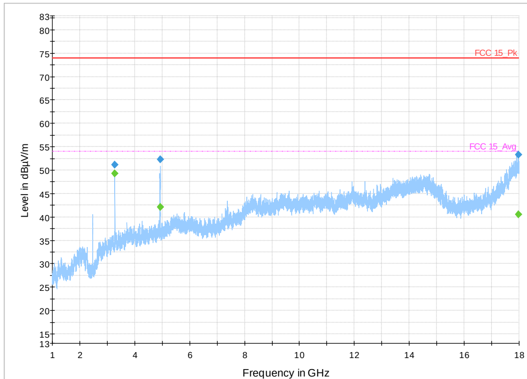
Plot 86. 1-18GHz 802.11b Mode, Channel 11
