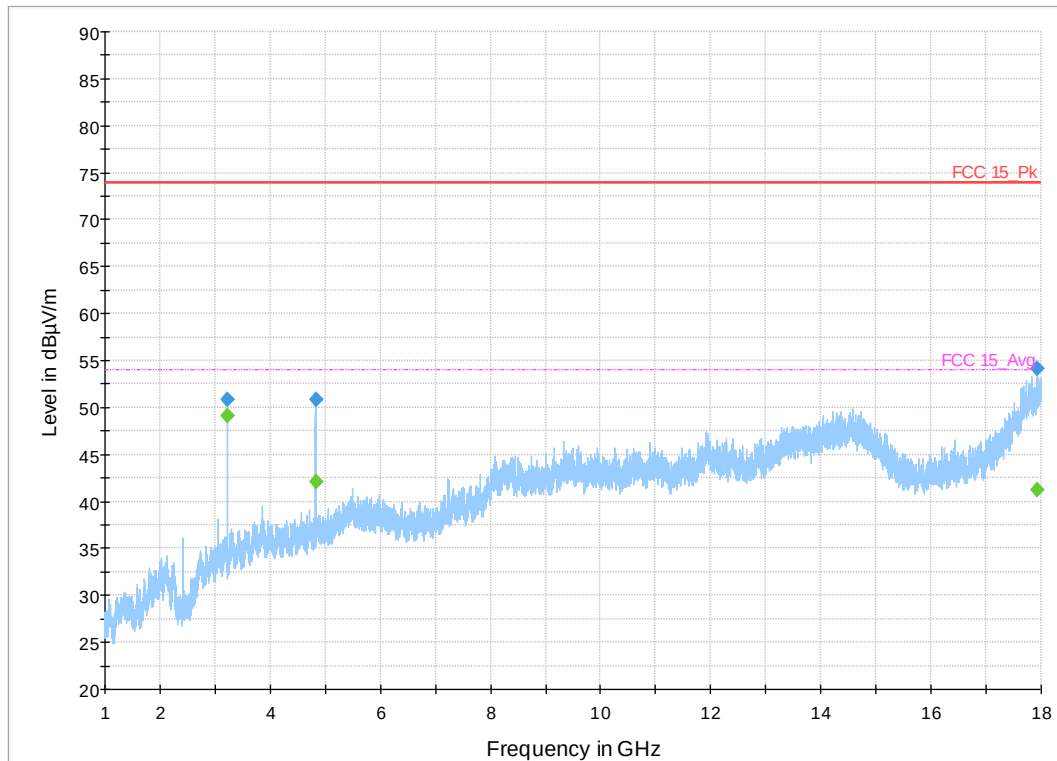
Plot 84. 1-18GHz 802.11b Mode, Channel 1
