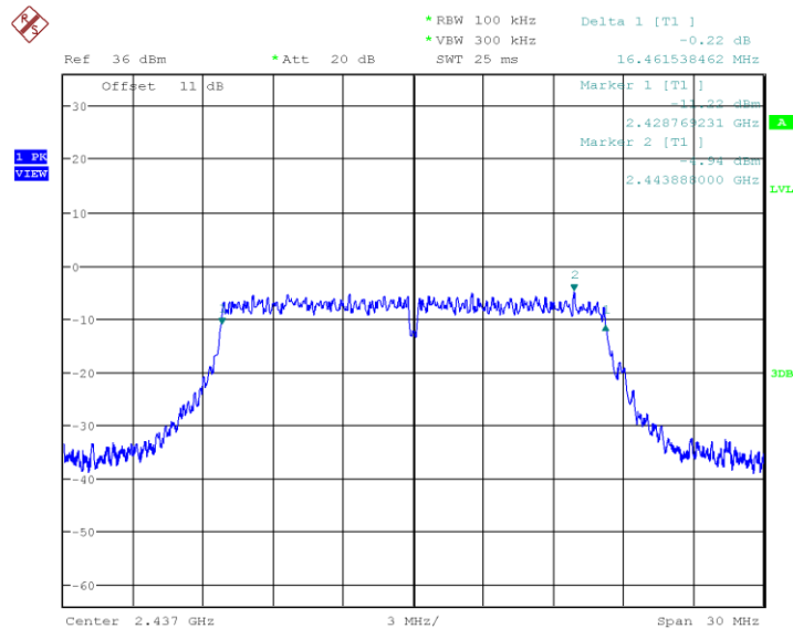
Plot 5. 802.11g(No HT), 2437MHz, 6dB Bandwidth
