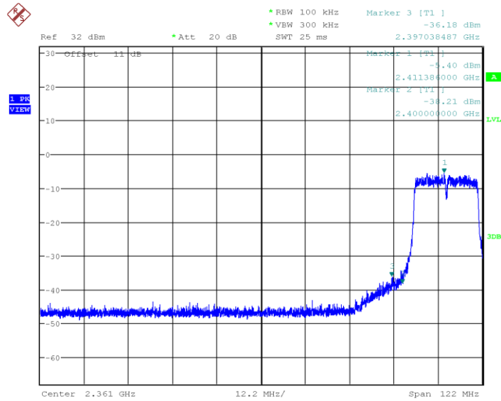
Plot 39. 802.11n HT20, 2412MHz Lower Band Edge
