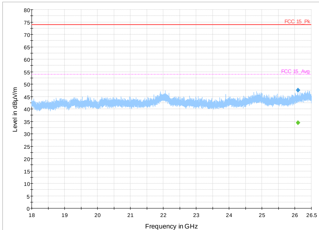
Plot 88. 18-26GHz 802.11b Mode, Channel 6
