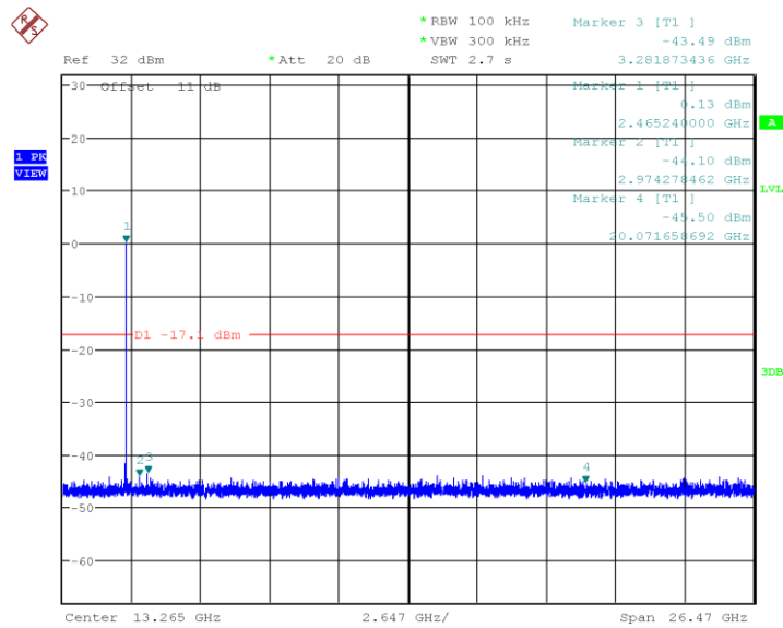
Plot 55. 802.11b CCK, 2462MHz, 30MHz-26.5GHz Non-restricted Out of Band
