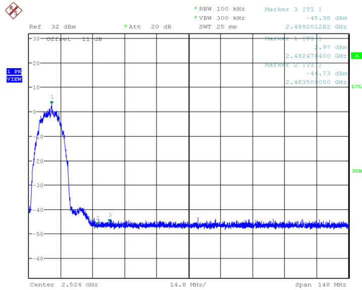
Plot 43. 802.11b CCK, 2462MHz Upper Band Edge
