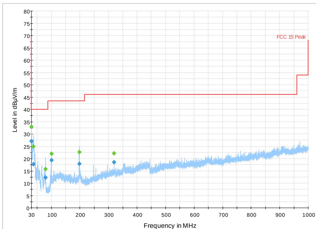
Plot 83. 30MHz-1GHz 802.11b Mode, Channel 6
