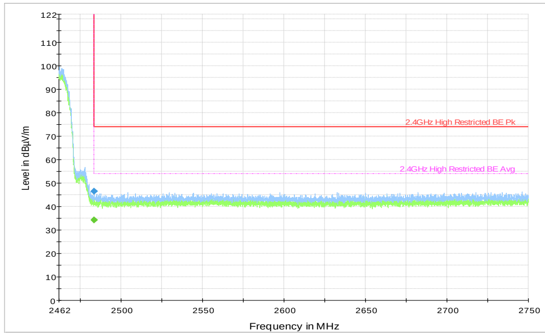
Plot 79. 802.11b CCK, 2462MHz, Upper Band Edge, Restricted
