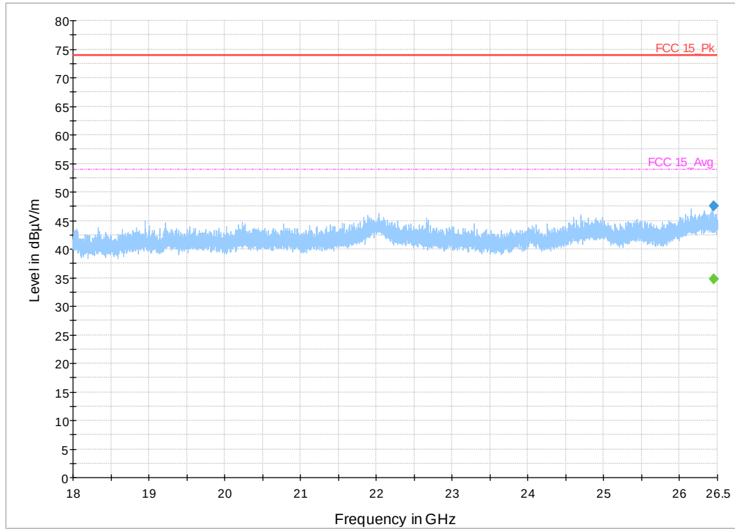
Plot 90. 18-26GHz 802.11n HT40 Mode, Channel 3
