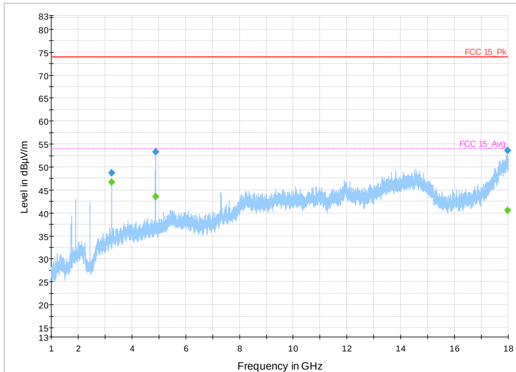
Plot 85. 1-18GHz 802.11b Mode, Channel 6
