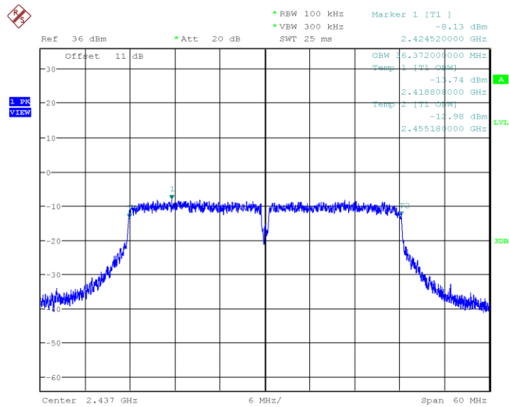
Plot 10. 802.11n(HT40), 2437MHz, 99% Bandwidth
