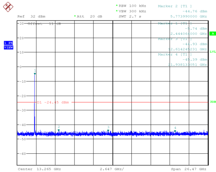
Plot 59. 802.11g No HT, 2437MHz, 30MHz-26.5GHz Non-restricted Out of Band
