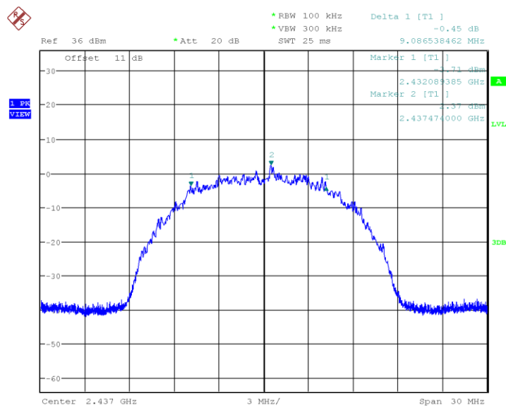
Plot 3. 802.11b(CCK), 2437MHz, 6dB Bandwidth
