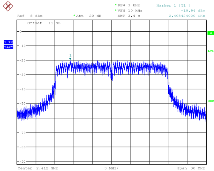
Plot 23. 802.11n HT20, 2412MHz PSD
