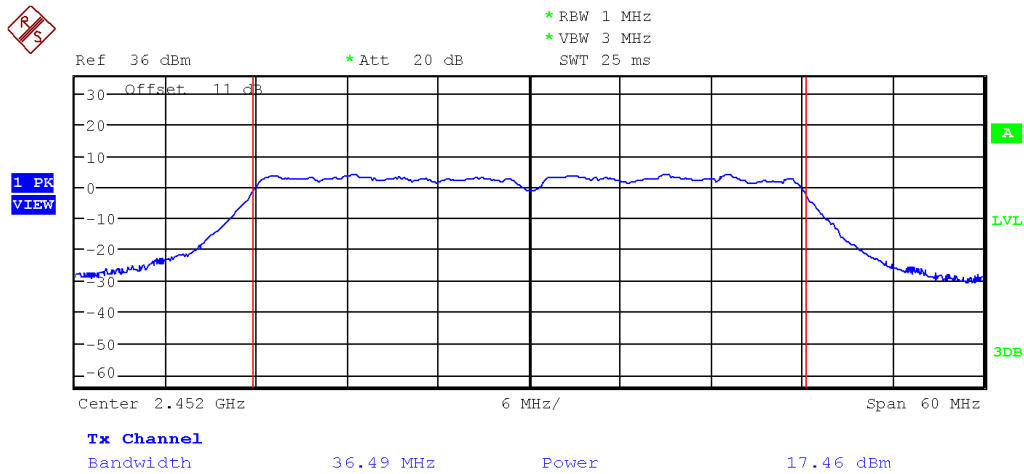
Plot 1. Maximum Conducted Power, 802.11n HT40 (MCS0) 13.5Mbps
