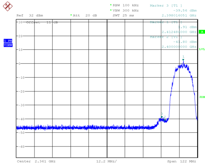
Plot 35. 802.11b CCK, 2412MHz Lower Band Edge
