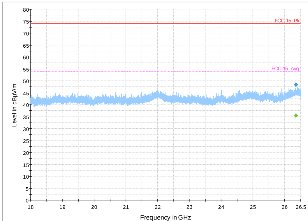
Plot 87. 18-26GHz 802.11b Mode, Channel 1
