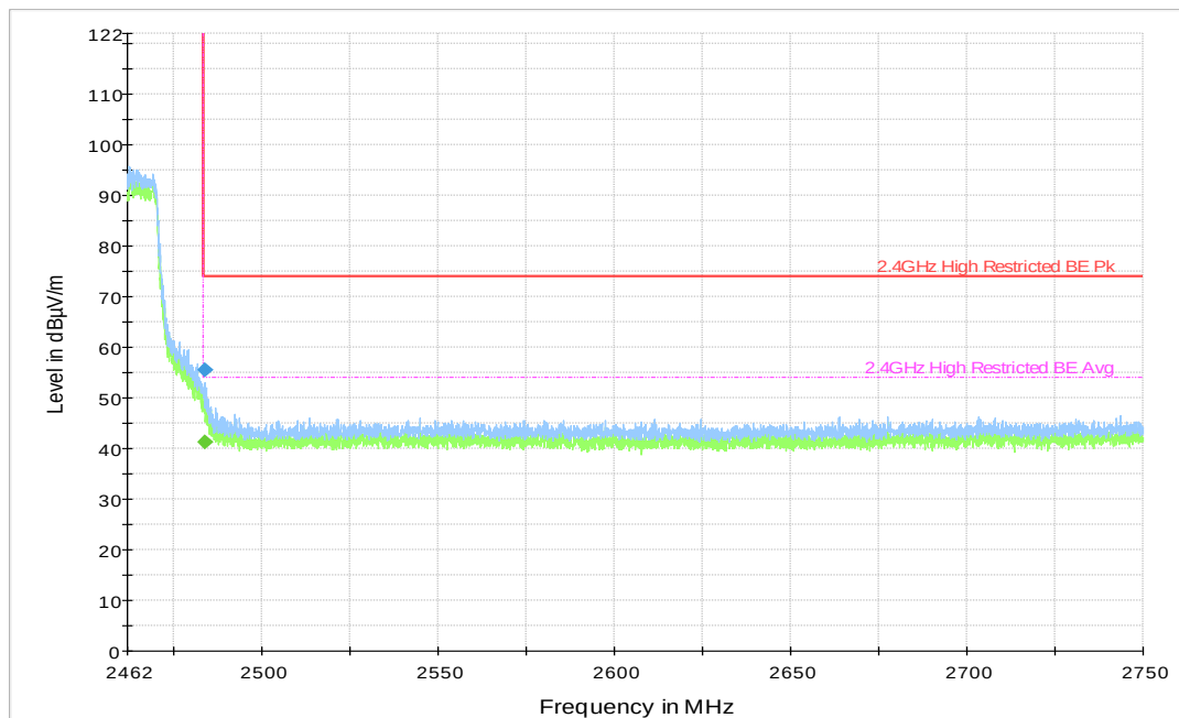
Plot 80. 802.11g No HT, 2462MHz, Upper Band Edge, Restricted
