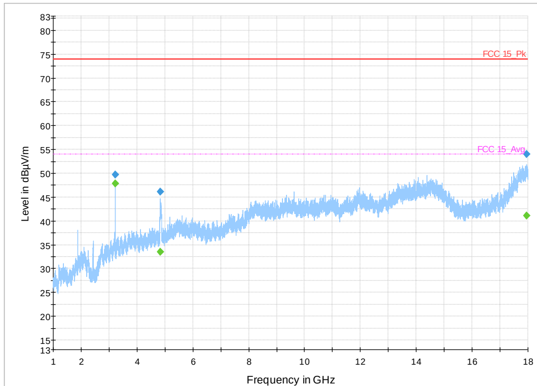
Plot 83. 1GHz-18GHz 802.11n HT40 Mode, Channel 3
