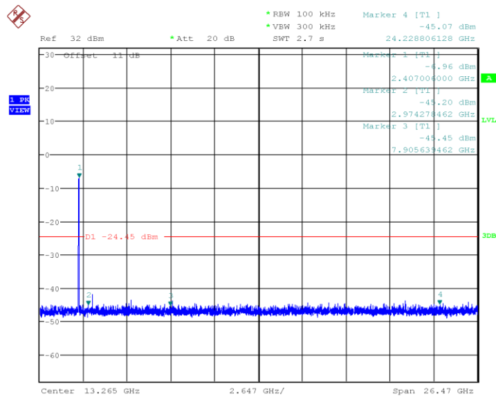
Plot 57. 802.11g No HT, 2412MHz, 30MHz-26.5GHz Non-restricted Out of Band
