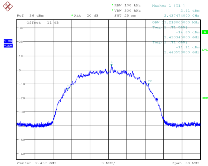
Plot 4. 802.11b(CCK), 2437MHz, 99% Bandwidth
