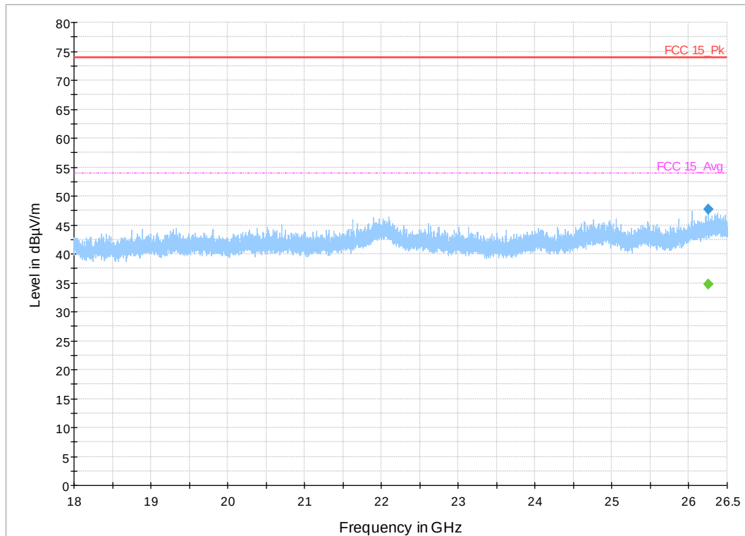
Plot 89. 18-26GHz 802.11b Mode, Channel 11
