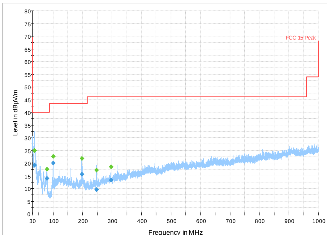
Plot 83. 30MHz-1GHz 802.11b Mode, Channel 1
