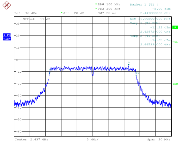
Plot 6. 802.11g(No HT), 2437MHz, 99% Bandwidth
