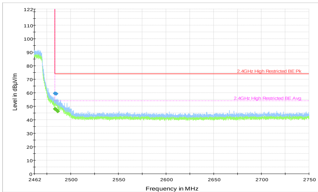
Plot 82. 802.11n HT40, 2452MHz, Upper Band Edge, Restricted
