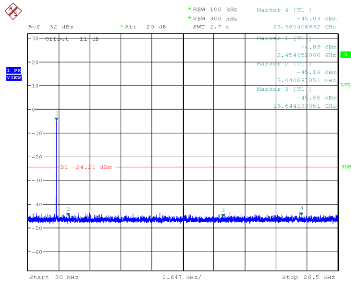
Plot 67. 802.11n HT20, 2462MHz, 30MHz-26.5GHz Non-restricted Out of Band
