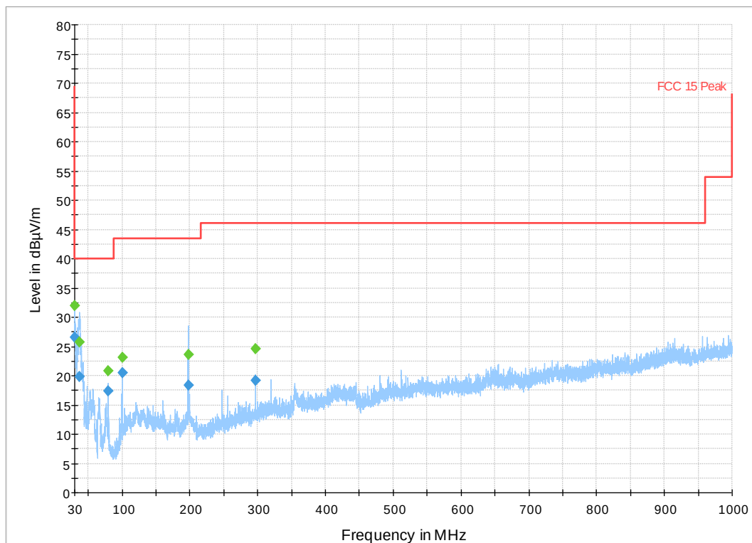
Plot 83. 30MHz-1GHz 802.11n HT40 Mode, Channel 3
