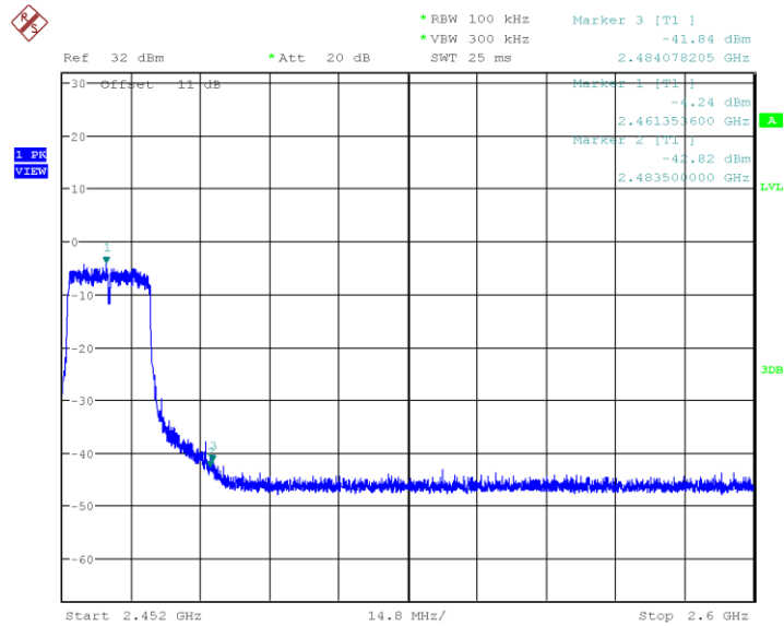
Plot 47. 802.11n HT20, 2462MHz Upper Band Edge
