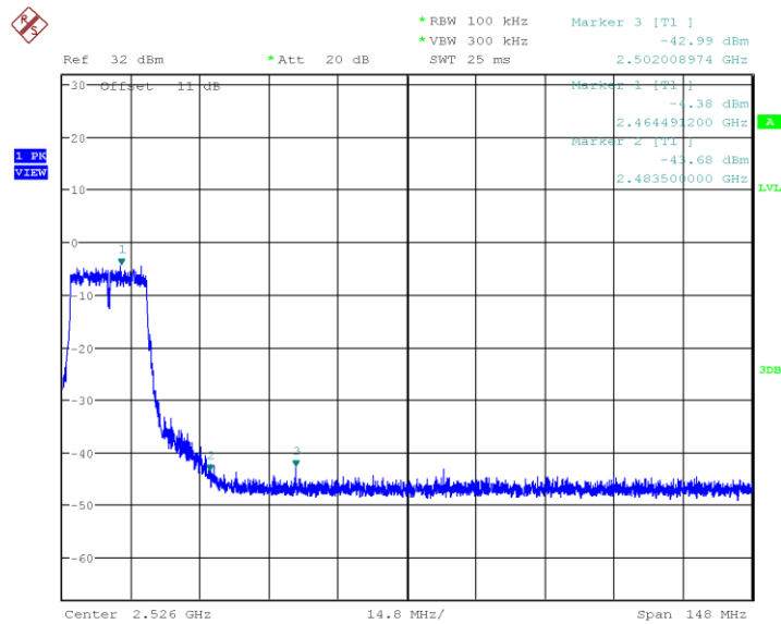
Plot 45. 802.11g No HT, 2462MHz Upper Band Edge
