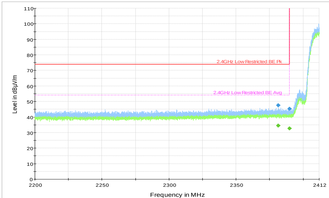
Plot 75. 802.11b CCK, 2412MHz, Lower Band Edge, Restricted
