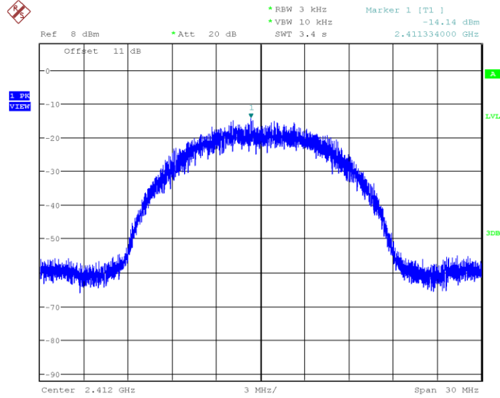
Plot 11. 802.11b CCK, 2412MHz PSD
