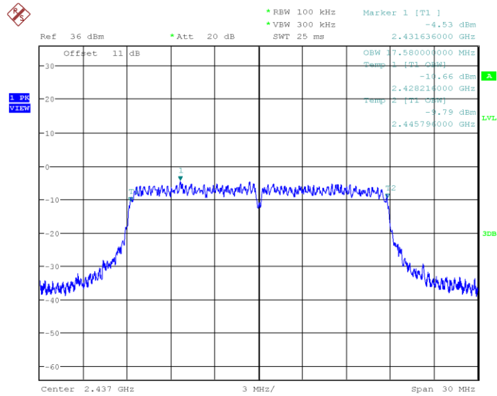
Plot 8. 802.11n(HT20), 2437MHz, 99% Bandwidth
