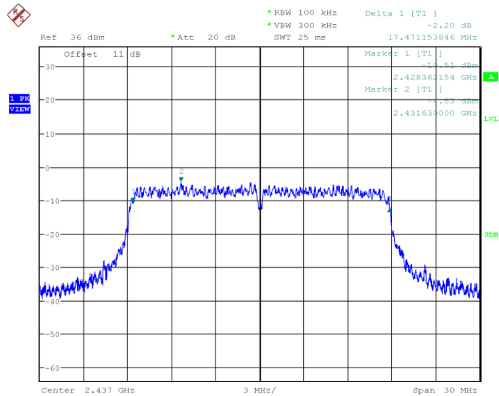
Plot 7. 802.11n(HT20), 2437MHz, 6dB Bandwidth
