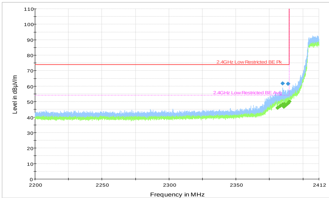
Plot 78. 802.11n HT40, 2422MHz, Lower Band Edge, Restricted
