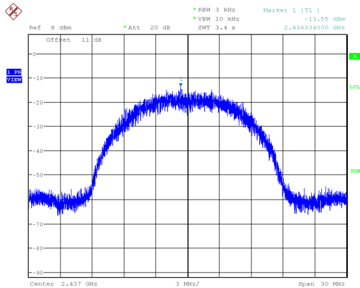
Plot 13. 802.11b CCK, 2437MHz PSD
