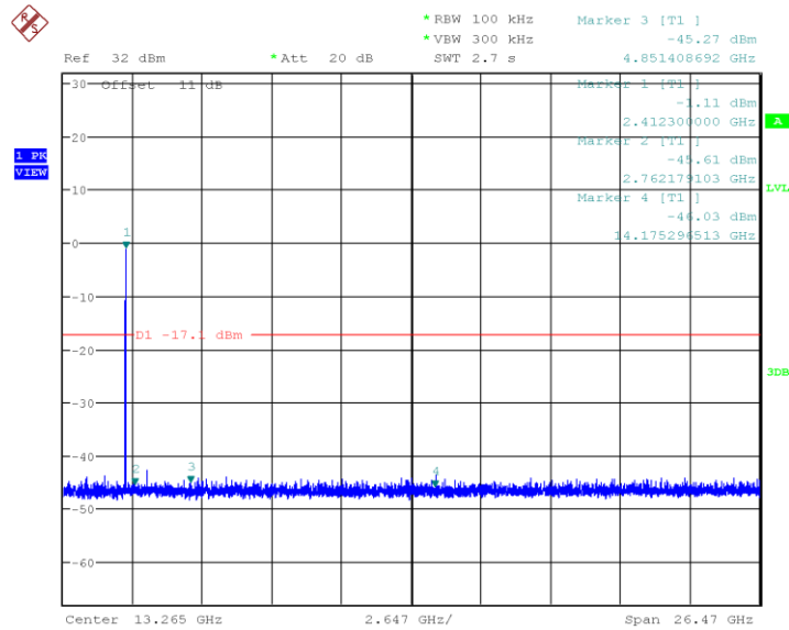
Plot 51. 802.11b CCK, 2412MHz, 30MHz-26.5GHz Non-restricted Out of Band
