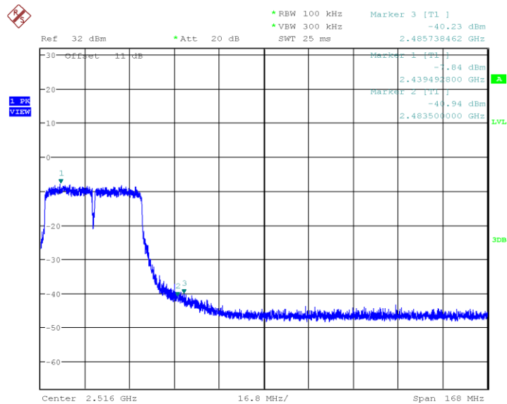
Plot 49. 802.11n HT40, 2452MHz Upper Band Edge
