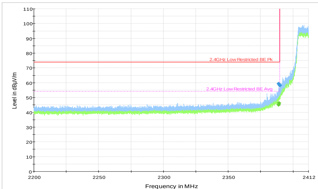
Plot 76. 802.11g No HT, 2412MHz, Lower Band Edge, Restricted
