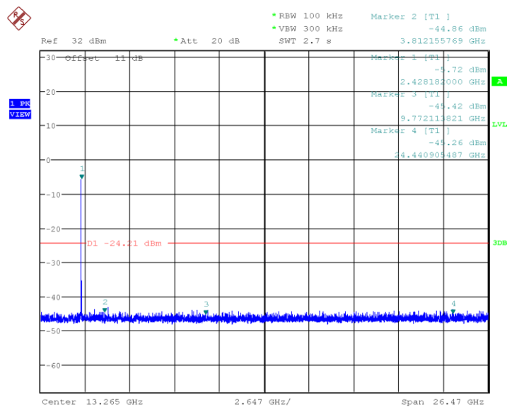
Plot 65. 802.11n HT20, 2437MHz, 30MHz-26.5GHz Non-restricted Out of Band
