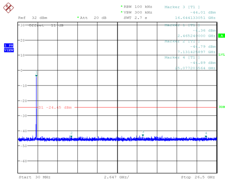
Plot 61. 802.11g No HT, 2462MHz, 30MHz-26.5GHz Non-restricted Out of Band
