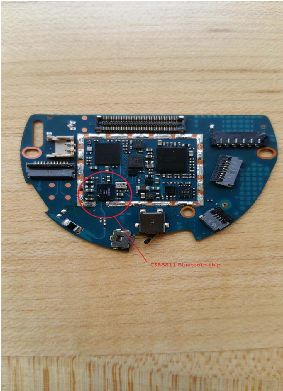
PCB TOP – SHIELD REMOVED
