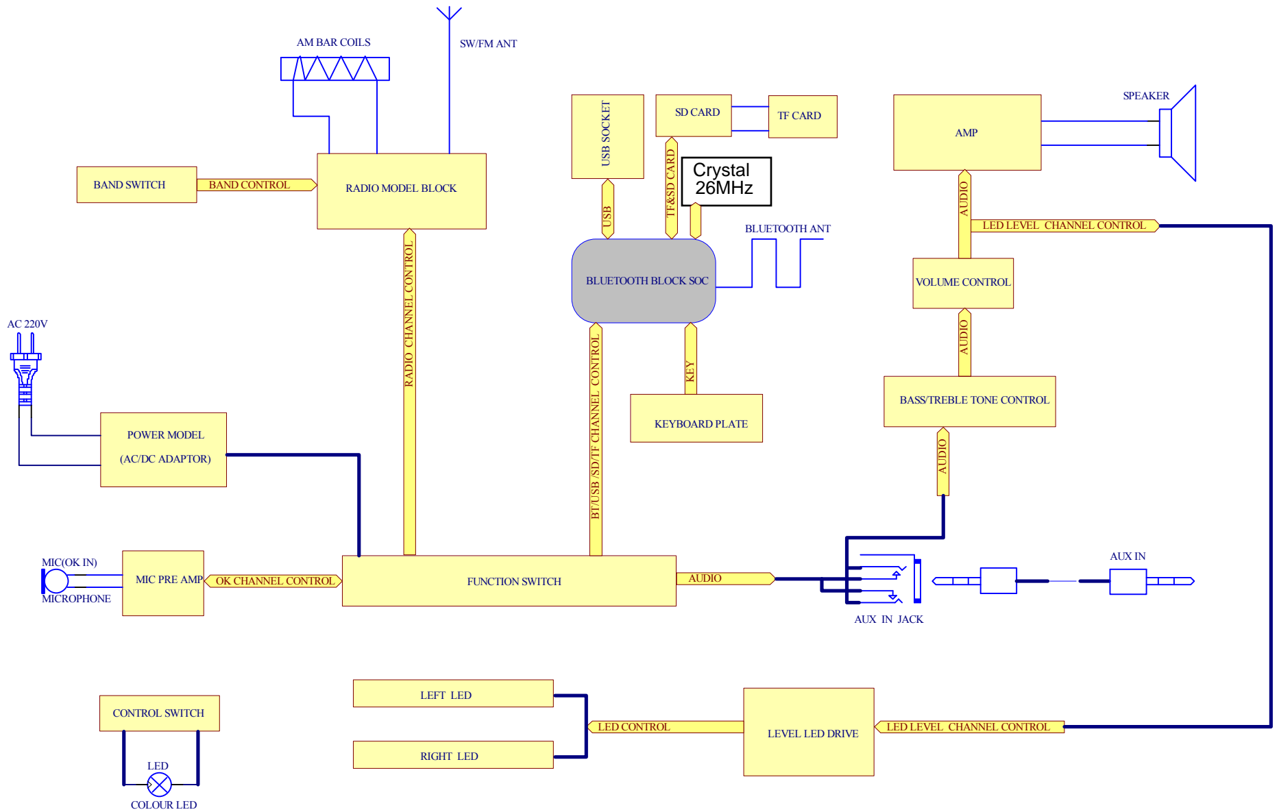
BLOCK DIAGRAM
