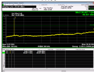
10th Harmonic of the fundamental frequency CH00 CH39 CH78
