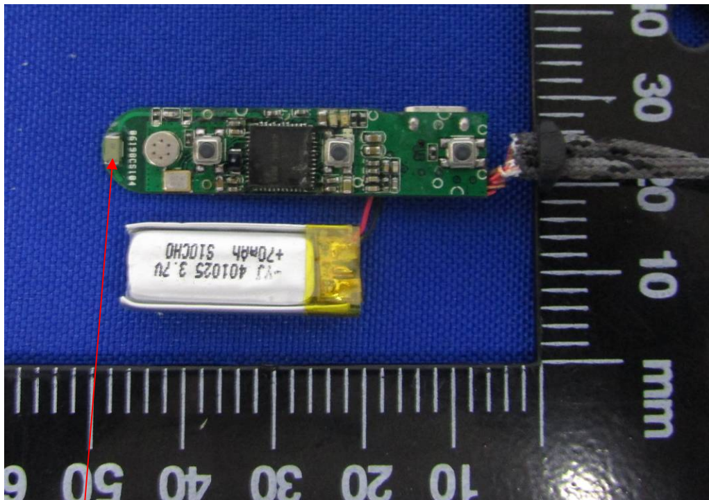
BT Antenna
