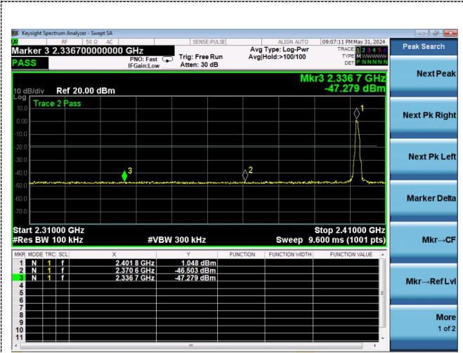
Left bandedge
